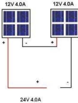
Series Connected Solar Panels
