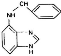
Benzylaminobenzimidazole
