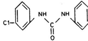
Chlorophenylphenylurea
