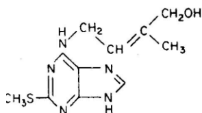
Methylthiozeatin
