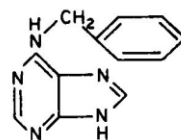
Benzyladenine (BA)
