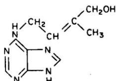
Zeatin
