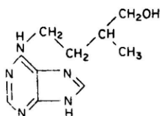
Dihydrozeatin
