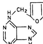
Kinetin
