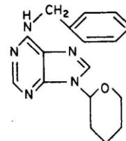
Tetrahydropyranylbenzyladenine (PBA)
