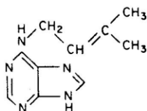
Dimethylallyladenine (DMAA)
