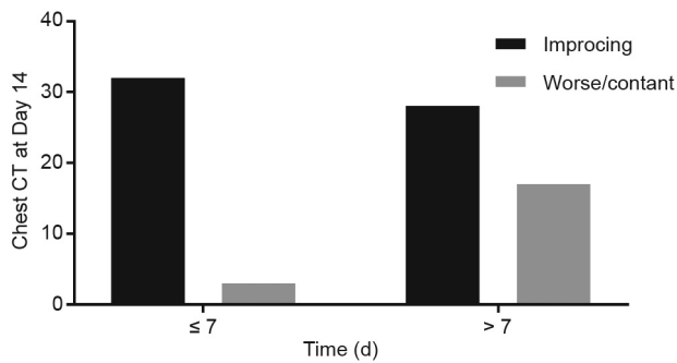
Fig. 4. Time of viral shedding and improving chest CT scan on Day 14 after treatment.
