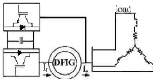
Figure 4 block diagram of self-excited DFIG
