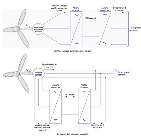
Figure 2 Circuit topologies for two types of generators found in variable-speed wind turbines
