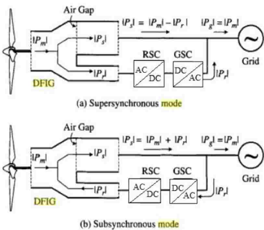
Figure 3 Power flow in DFIG wind energy conversion system
