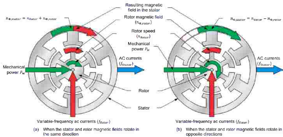
Figure 1 Interaction between the rotor speed and the frequency of the rotating magnetic field created in the rotor windings of a doubly-fed induction generator
