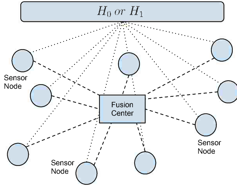
FIGURE 1.1: Architecture of a CRN
