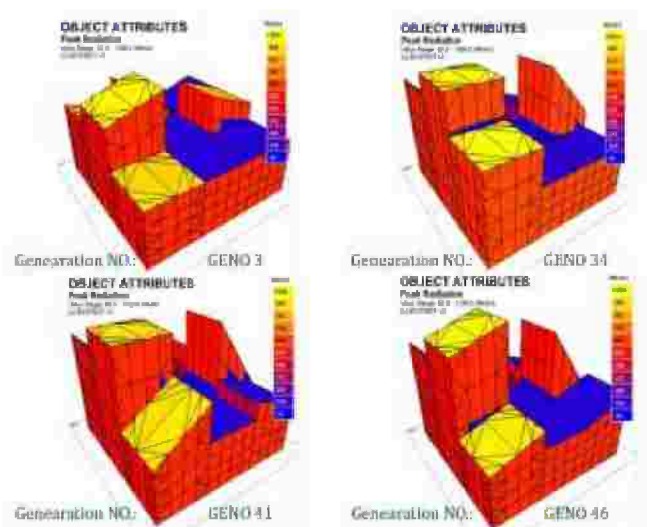
Figure (6- 12): Cairo's best generations – Grasshopper – Geco – Galapagos
