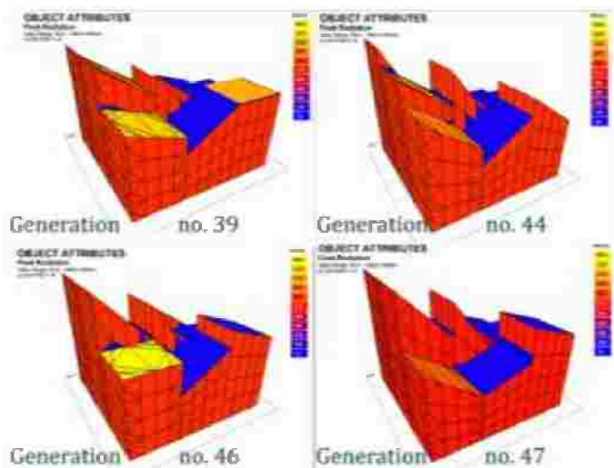
figure (6- 14): Alexandria's best generations – Grasshopper –Geco – Galapagos Source: Researcher 2014
