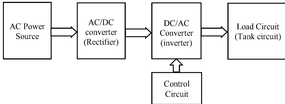
Figure 1.3 Layout of basic induction heating system
