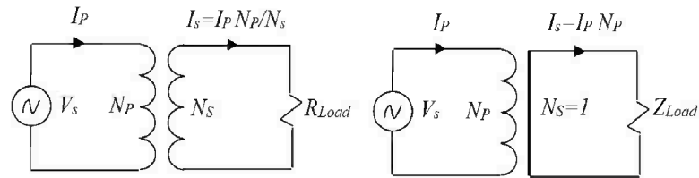
Figure 1.1 Basic concepts of induction heating (a) Transformer circuit. (b) Short circuit secondary circuit.
