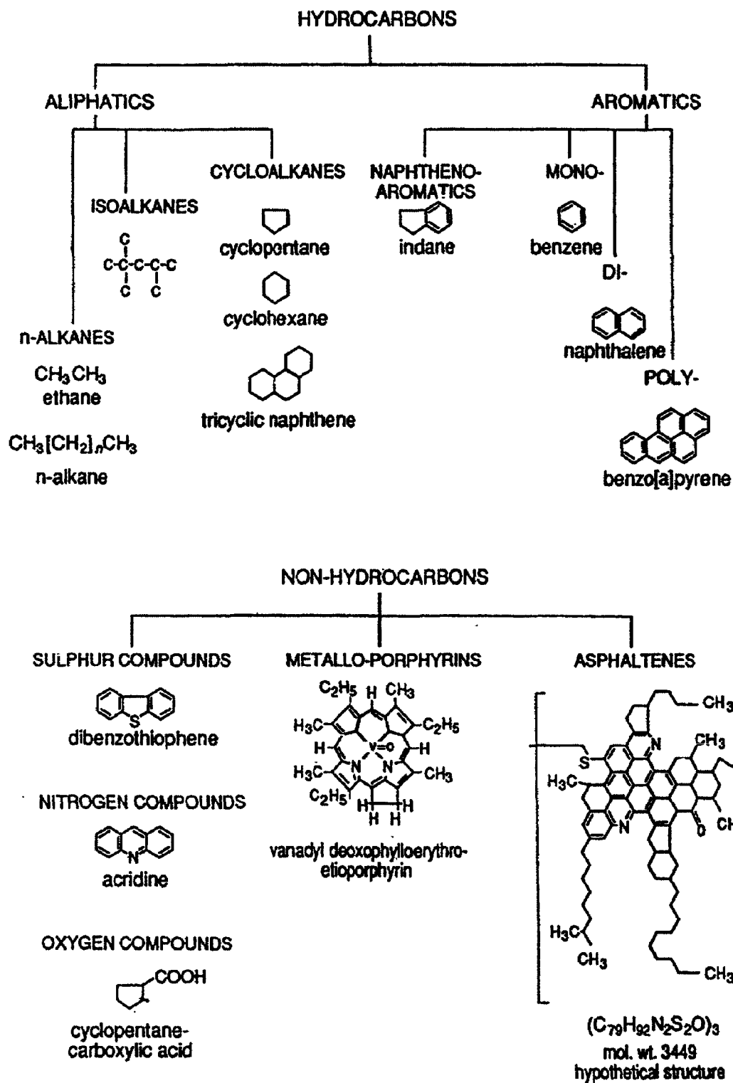
Fig.(1): Examples of the chemical structure of some common components of crude oil
