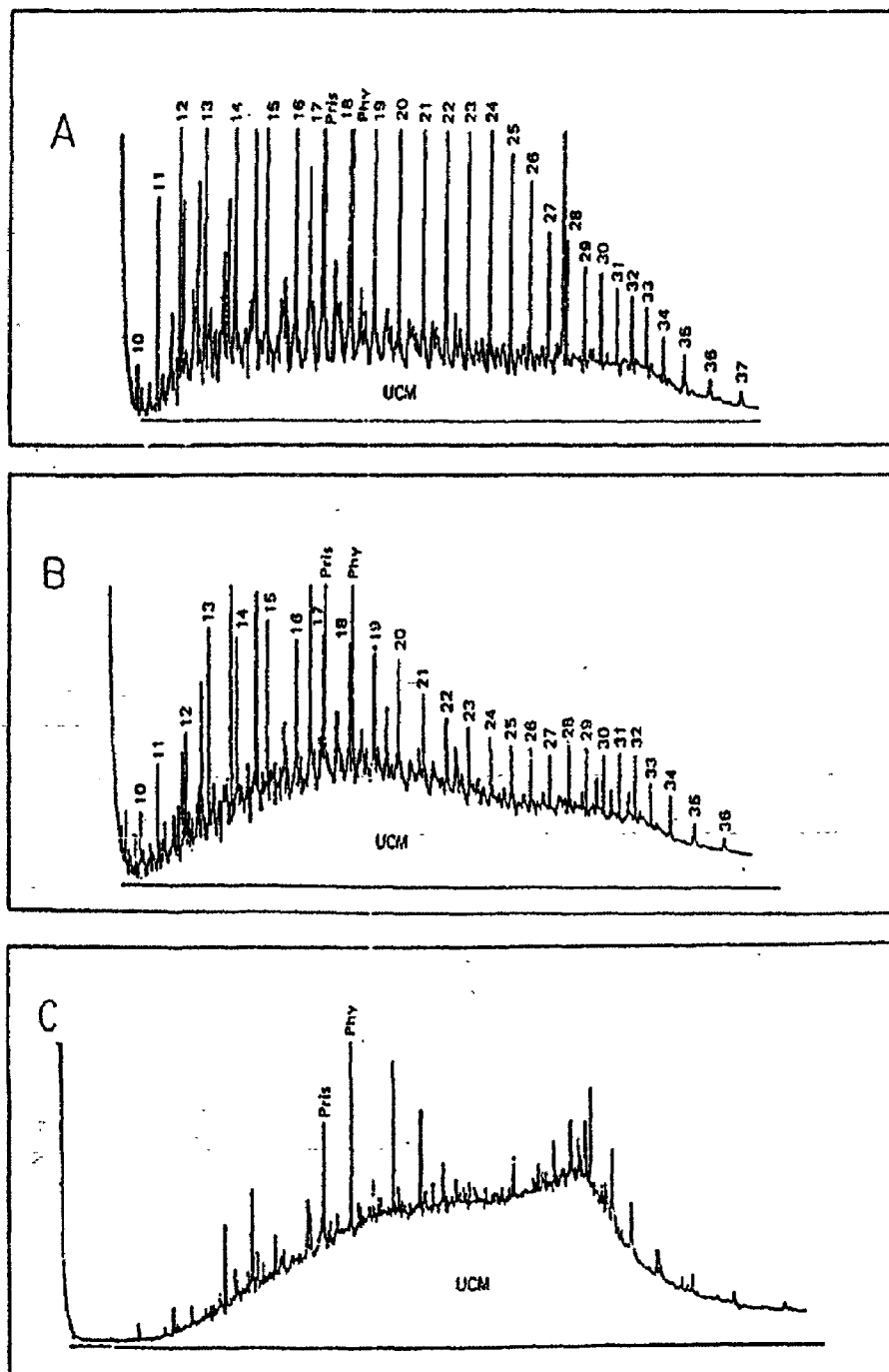
Fig.(3): Gas chromatograms for (A) waxy crude oil, (B) weathered and (C) very highly weathered crude oil.
