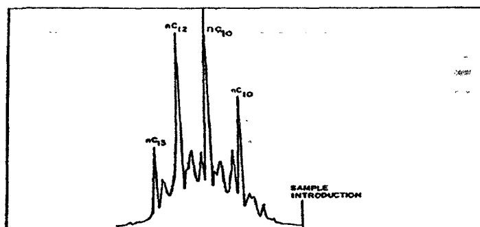
Fig.(6): Gas chromatogram for light petroleum fraction.
