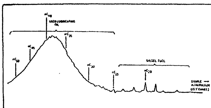
Fig.(5): Gas chromatogram for used lubricating oil.
