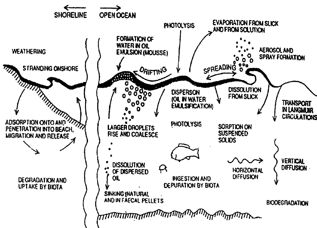
Fig.(2): Schematic diagram of oil spill processes at sea and shorelines
