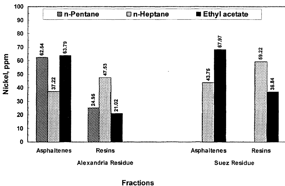
Figure-9: Distribution of the Nickel in the Asphaltenes and Resins in the Studied Vacuum Residues.
