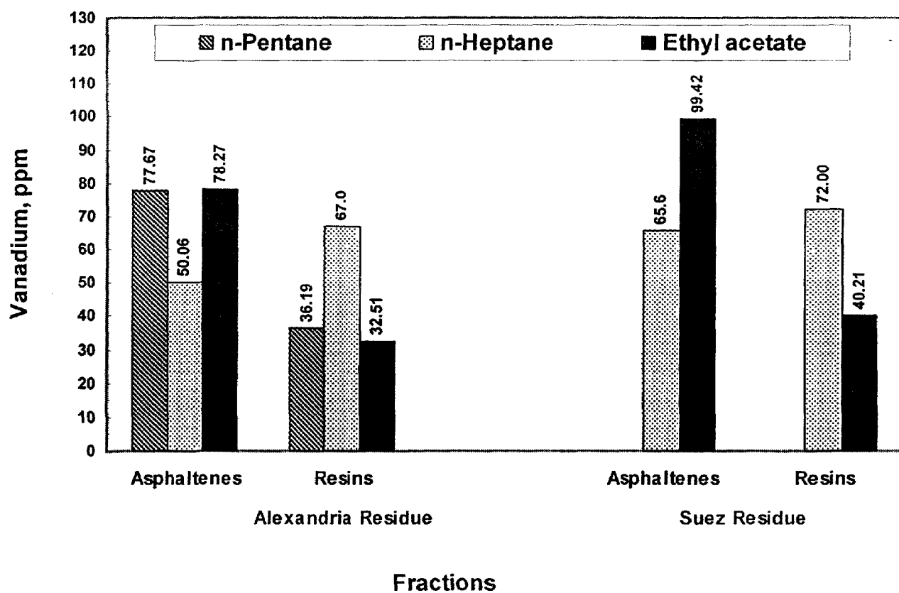
Figure-10: Distribution of the Vanadium in the Asphaltene and Resins in the Studied Vacuum Residues.
