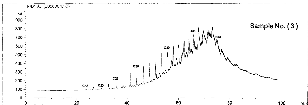
Figure-13:Gas chromatogram of Saturates Separated from Alexandria Residue Using Ethyl Acetate
