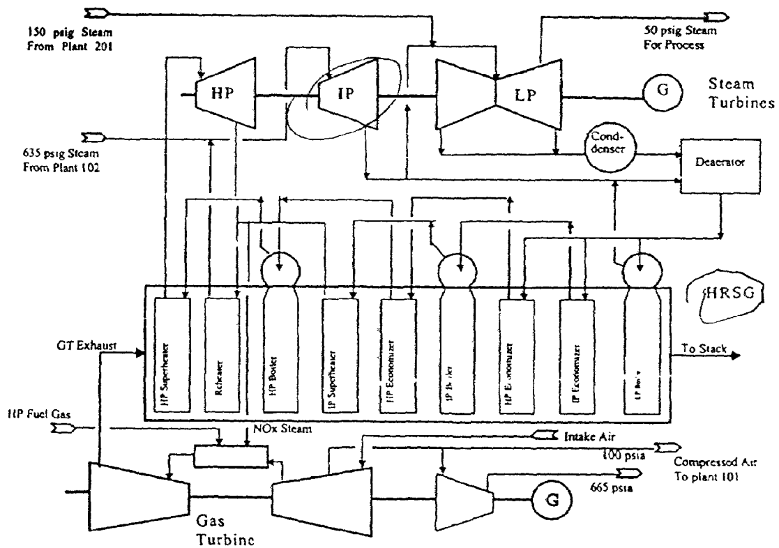
Figure 4-6 Block Flow Diagram - Combined Cycle Plant
