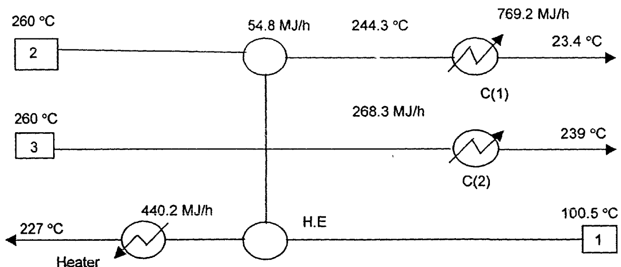
Figure (4-8) Actual gride diagram for the existing heat exchangers network of liquid phase Fischer-Tropsch Q_H = 440.2 \text{ MJ/h} and Q_C = 1037.5 \text{ MJ/h}
