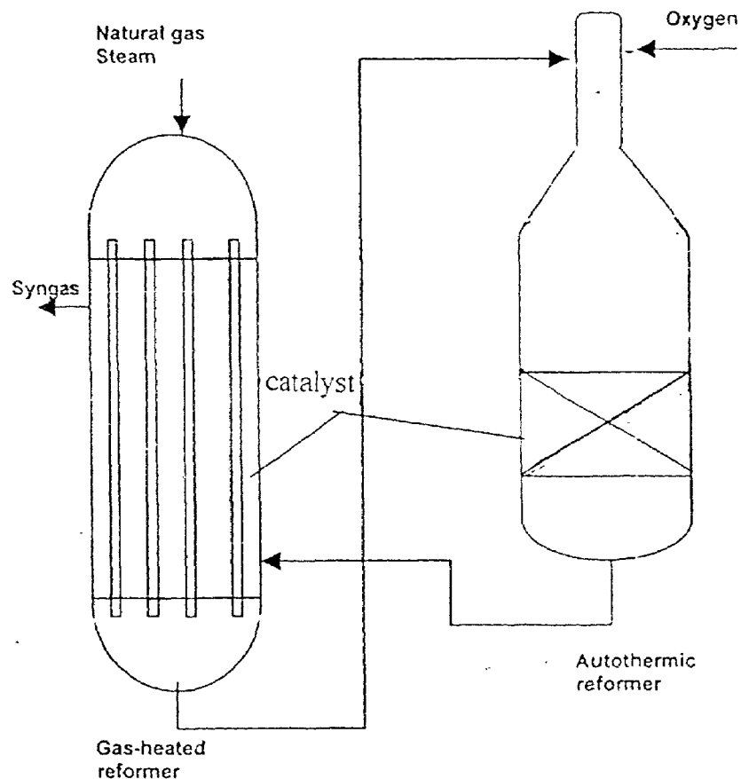
figure (4-1 ) ICI Combined- Reforming
