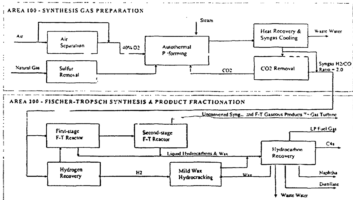
Figure 4-5 Once-Through Fischer-Tropsch (F-T) Design with Power Co-Production (Overall Process Configuration)
