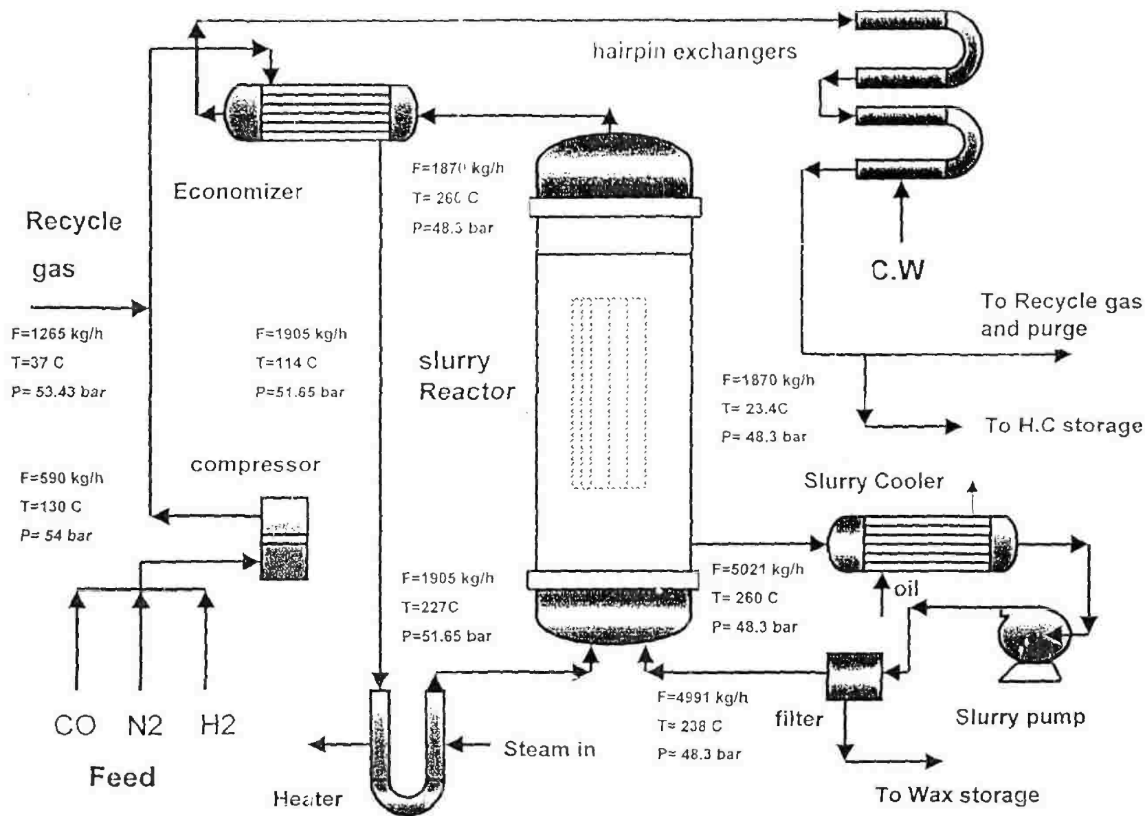
Fig(7-c) Simplified flow diagram for the AFDU pilot unit
