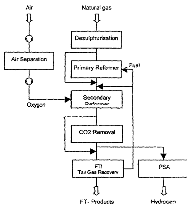
Figure 4-3 Lurgi Combined Reforming for F-T Synthesis
