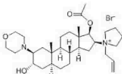
Figure (1): Rocuronium chemical structure
