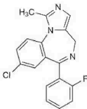
Figure (2): Midazolam chemical structure
