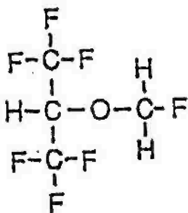
Figure (4): Sevoflurane chemical structure (32)
