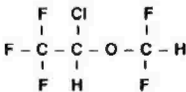
Figure (3): Isoflurane chemical structure
