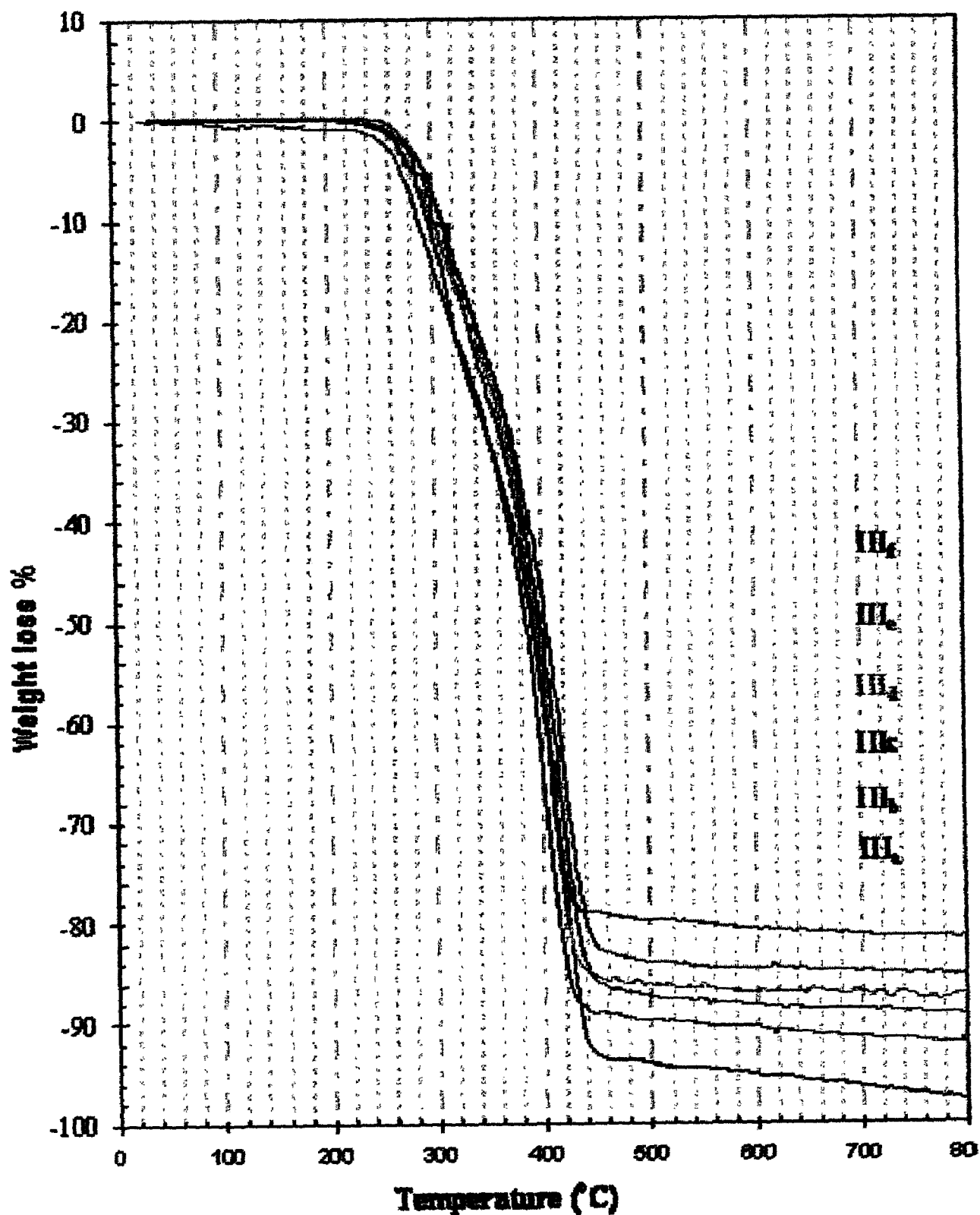
Figure 11: TGA thermographs under argon atmosphere for PU-organoclay composites III.4 (Tyr-MMT)
