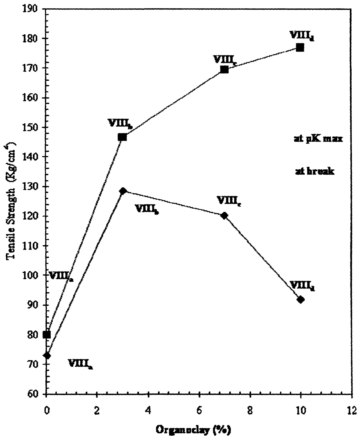
Figure 18: Tensile strength versus organoclay content for PU/ vinyl monomer-MMT nanocopolites (VIII a-d ) at pK max and at break
