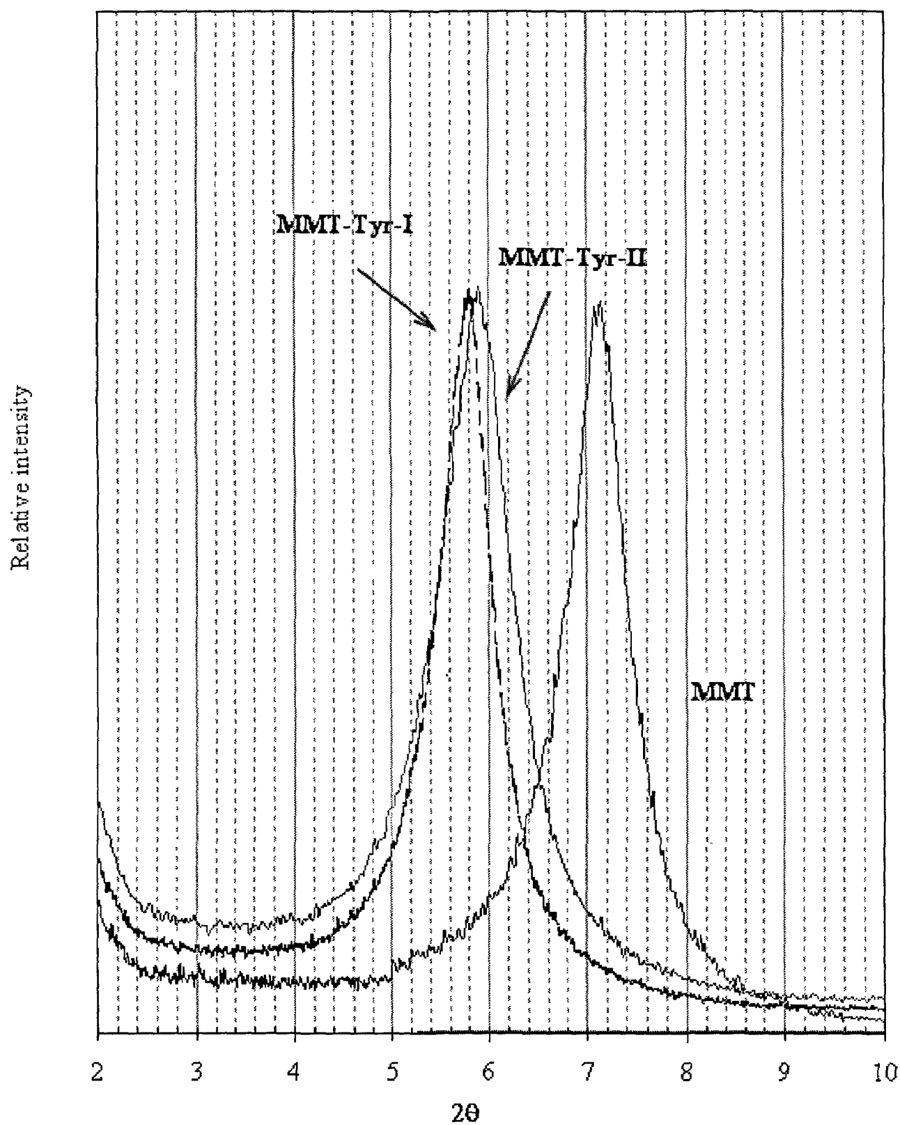
Figure 24 : The X-ray diffraction patterns of Tyr – MMT ( I_a ) first and second treatmen
