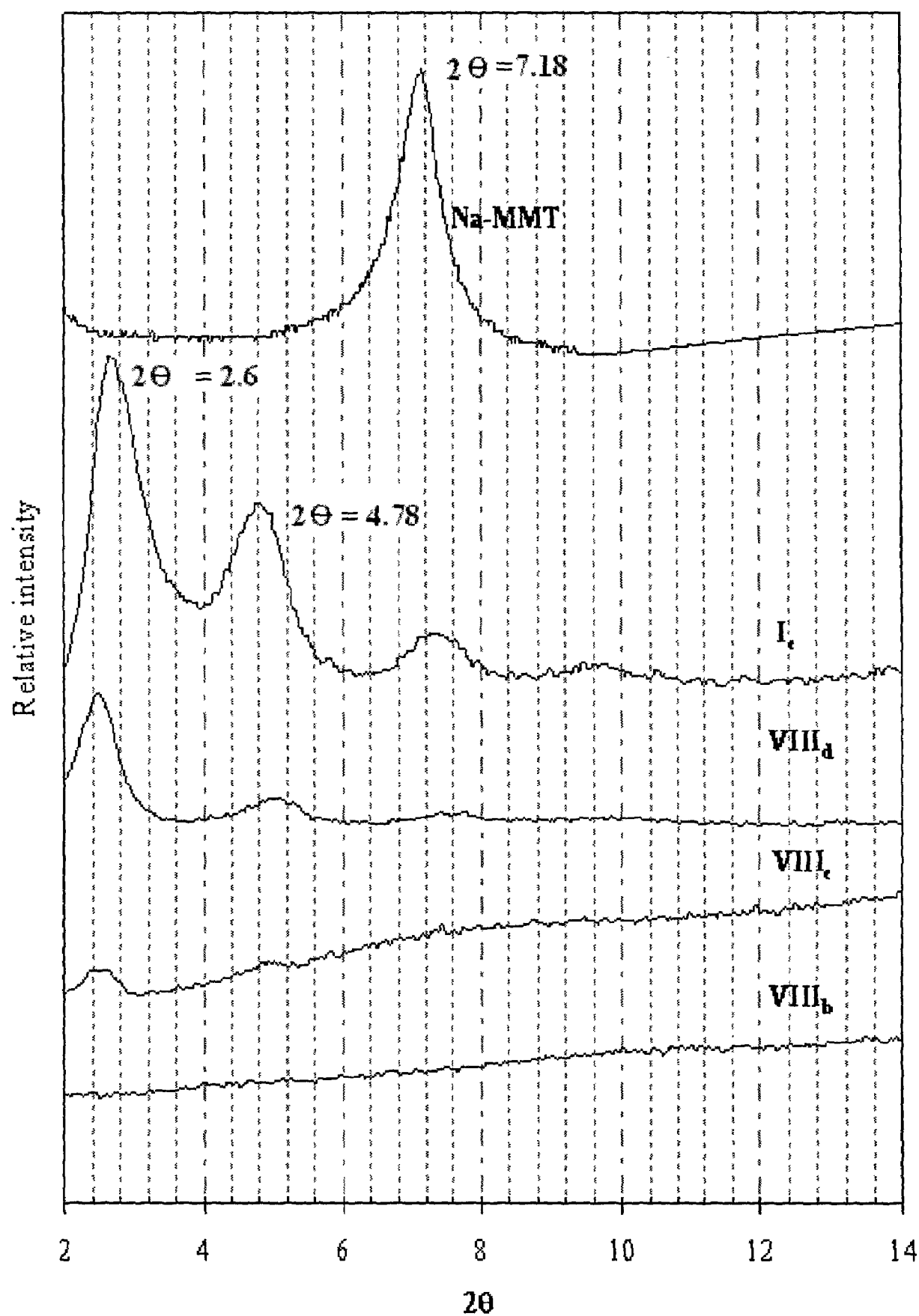
Figure 28: XRD pattern for Na-MMT, I_t and VIII b-d
