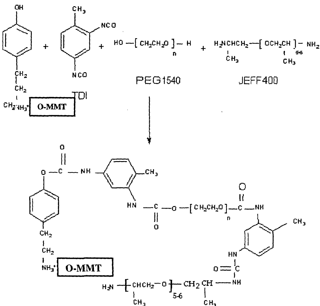
Scheme 2: Preparation of PU/Tyr-MMT composites III a-f
