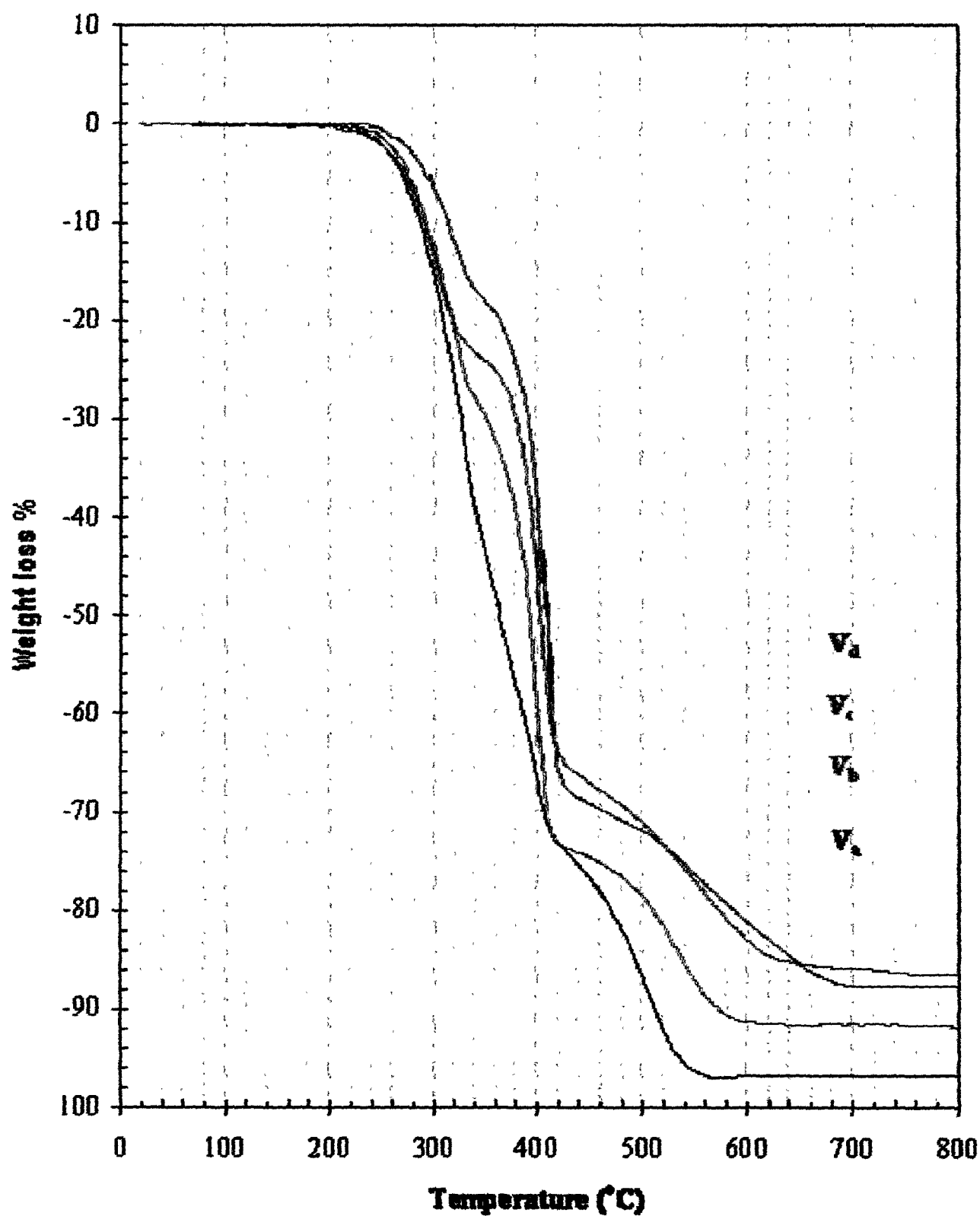
Figure 12: TGA thermographs for the PU-organoclay samples V a-d in atmospheric air
