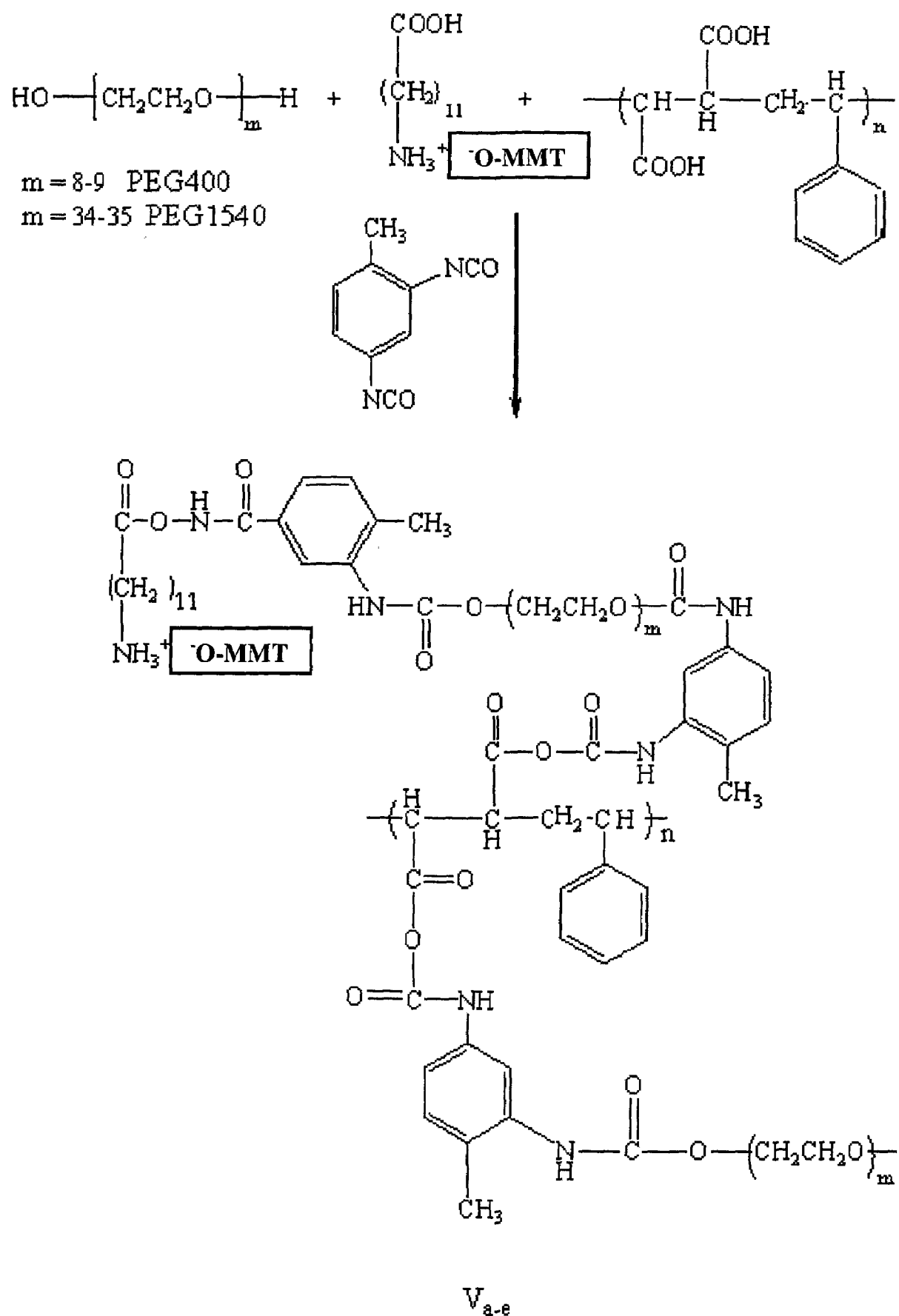
Scheme 4: Preparation of PU-MMT composites V_{a-e}
