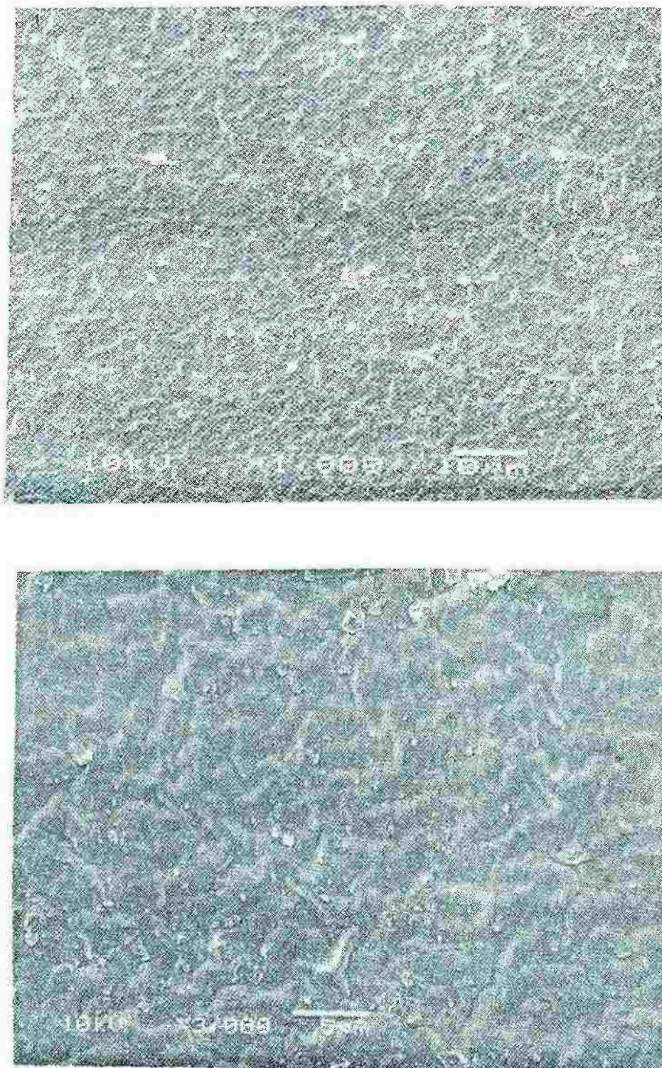
Figure 35: SEM micrograph of PU/ vinyl monomer-MMT, 3 wt. % (VIII b ) at different magnification
