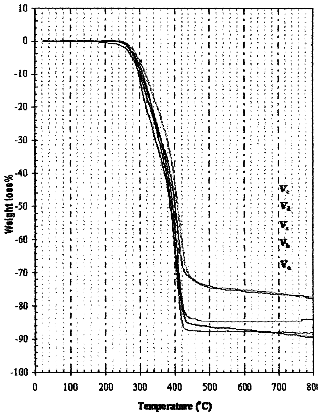
Figure 13: TGA thermographs for the PU-organoclay samples V_{1-5} under argon atmosphere
