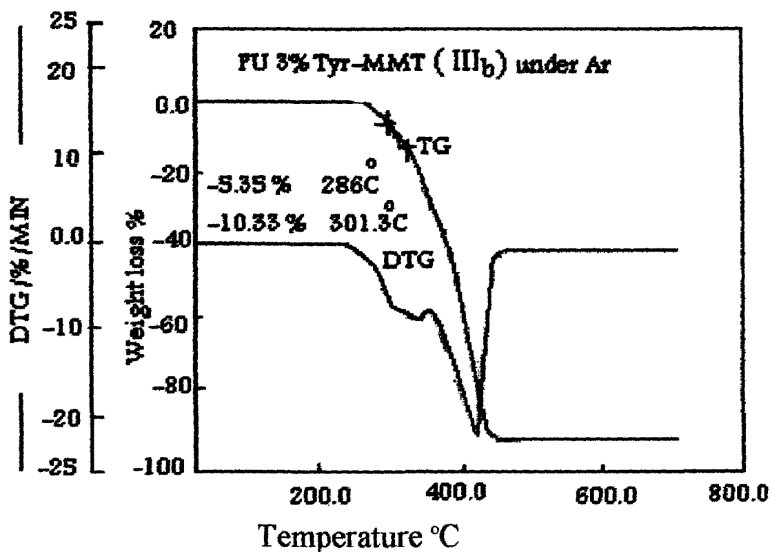
Figure 15: TGA and DTG of III b and III c
