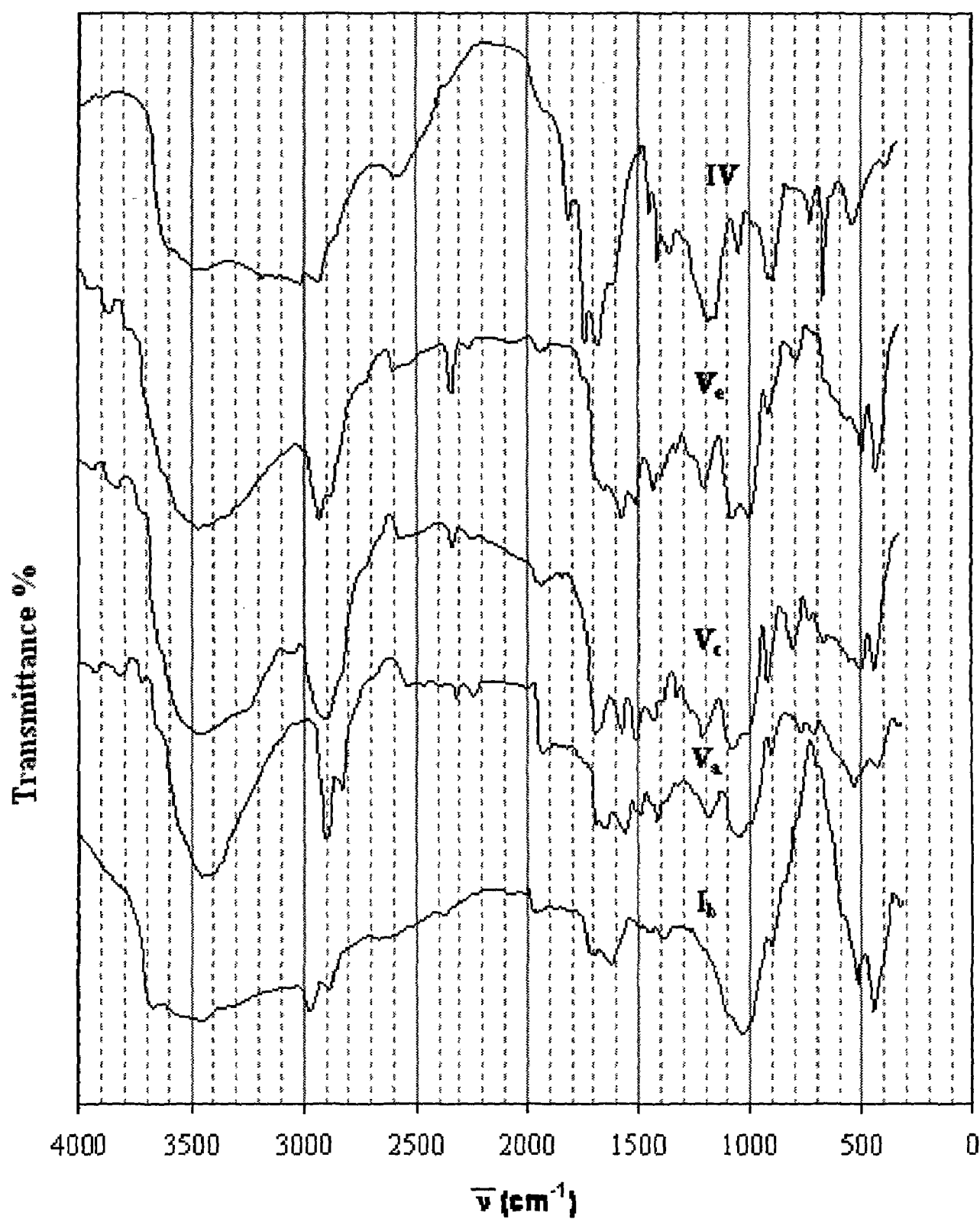
Figure 8: IR spectra for organoclay I b , copolymer IV and PU-organoclay V a, c, e
