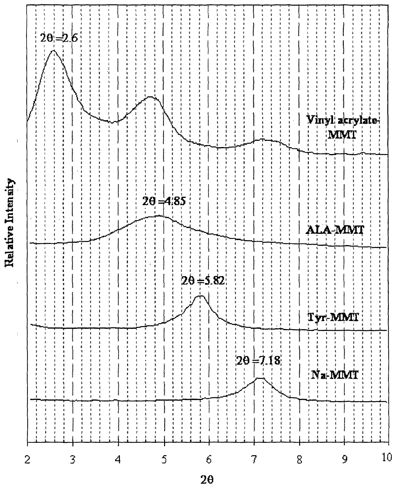
Figure 25: The X-ray diffraction patterns of Tyr-MMT ( I_1 ), ALA-MMT ( I_2 ), vinyl acrylate-MMT ( I_3 ) and Na-MMT
