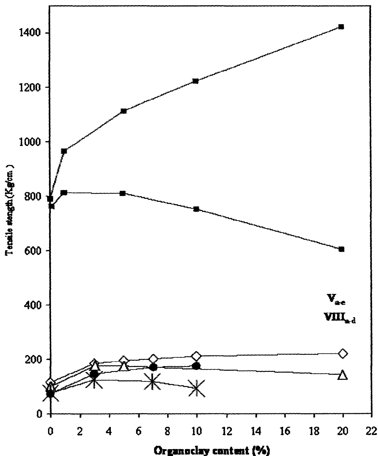
Figure 22: Tensile strength versus organoclay content for PU-organoclay hybrids at pKmax (—) and at break (—)
