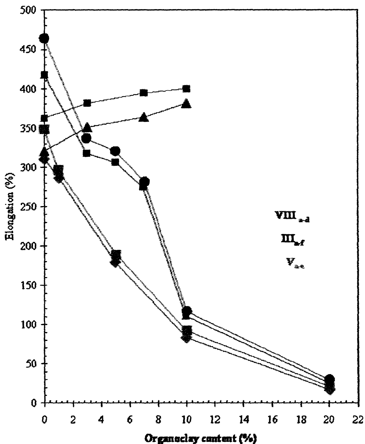
Figure 23: Elongation versus organoclay content for PU-organoclay hybrids at pKmax (—) and at break (---)
