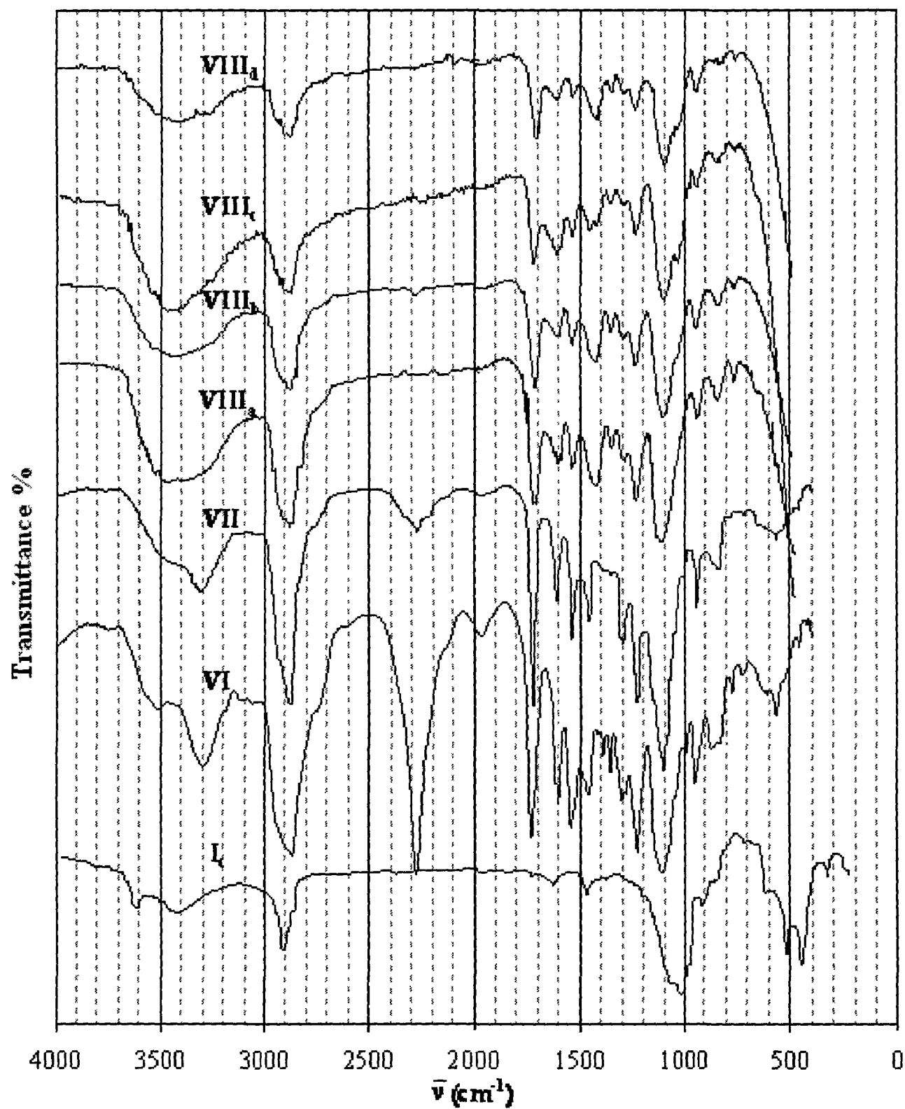
Figure 9: IR spectra of Ic , VI , VII and VIII a-d
