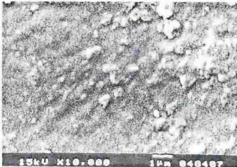
Figure 30: SEM micrograph for PU/T yr-MMT nanocomposite 5 wt. % (IIIc) at different magnifications
