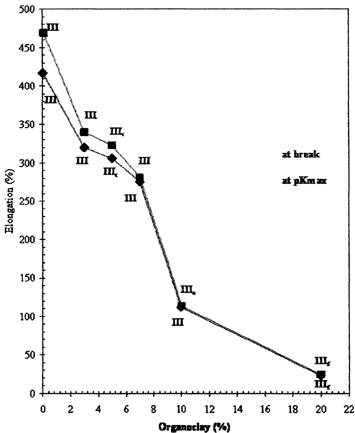
Figure 19: Elongation versus organoclay content for PU/ Tyr -MMT nanocomposites ( III_{0.5} ) at pK_{max} and at break
