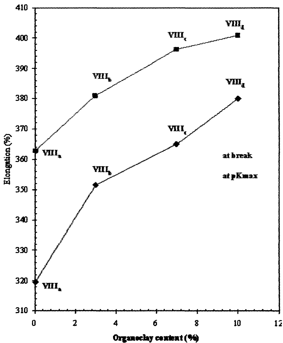
Figure 21: Elongation versus organoclay content for PU/ vinyl monomer-MMT nanocomposites (VIII a-d ) at pKmax and at break.
