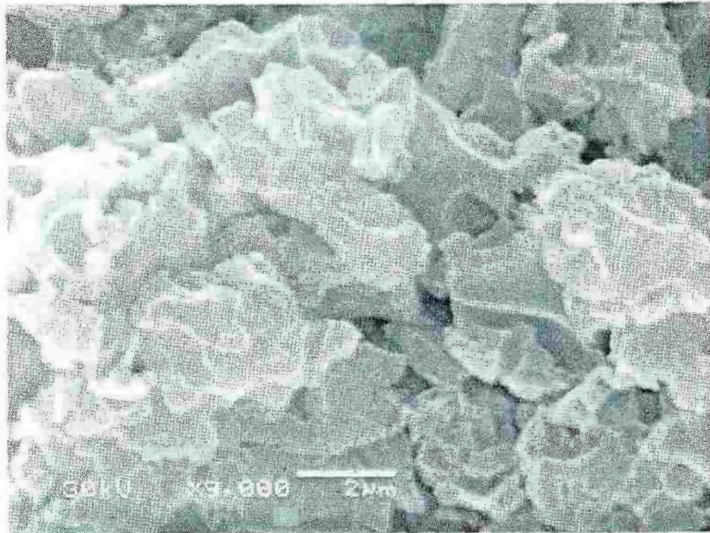
Figure 29a: SEM micrograph for PU/ Tyr-MMT, 3wt. % (III b )
