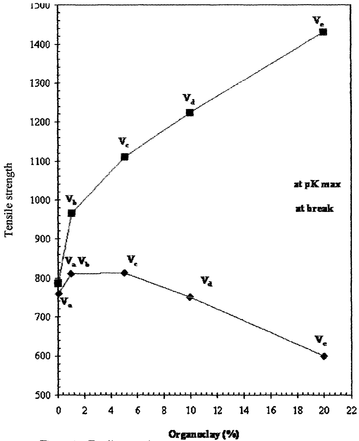
Figure 17: Tensile strength versus organoclay content for PU/SMA-ALA-MMT nanocomposites( V_{a-e} ) at pKmax and at break
