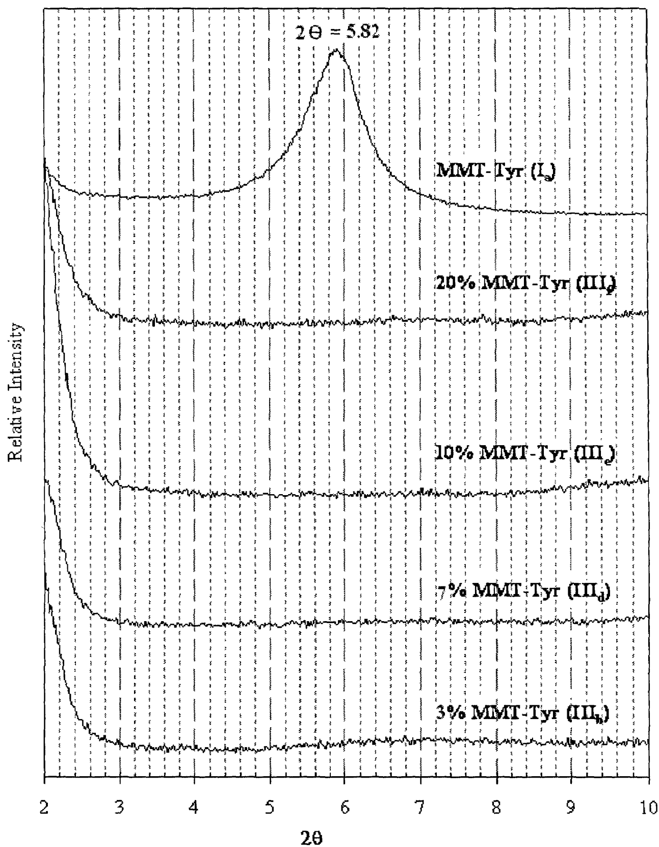
Figure 26: XRD pattern for Na-MMT, organoclay (I a ) and III b,d,f
