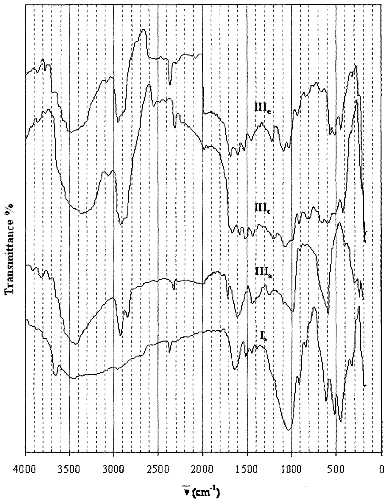
Figure 7: IR spectra for organo clay Ia, and PU-Tyr-MMT III a,c,e
