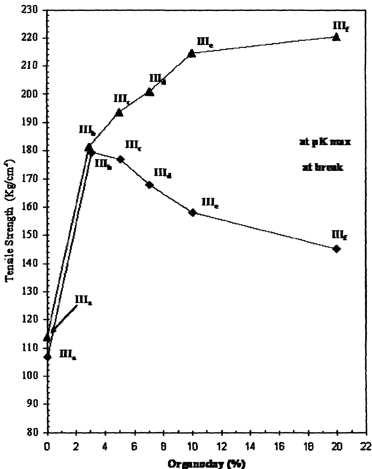
Figure 16: Tensile strength versus organoclay content for PU/Tyr-MMT nanocomposites (III a-f ) at pKmax and at break
