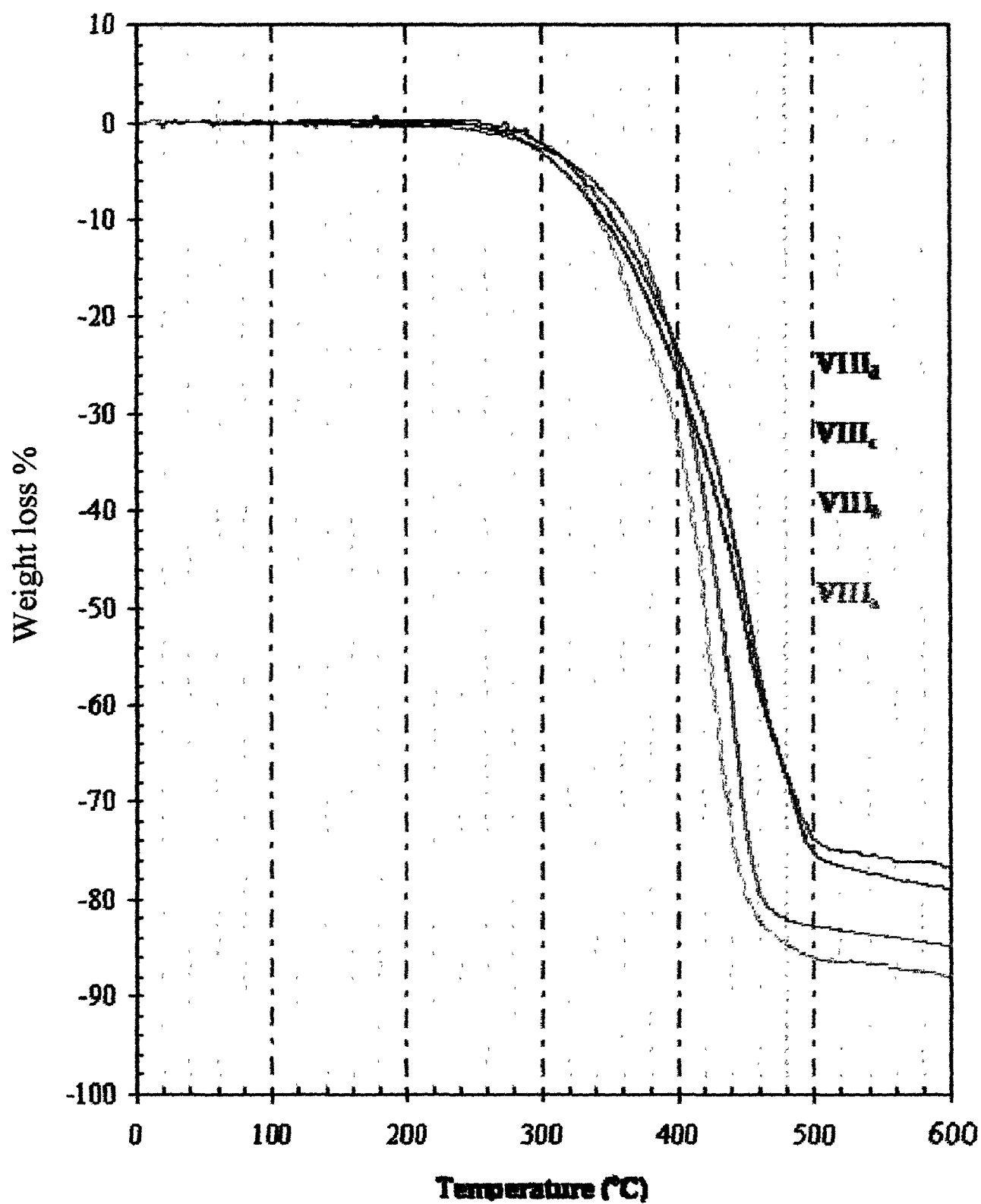
Figure 14: TGA Thermographs of VIII_{2-4} under nitrogen atmosphere
