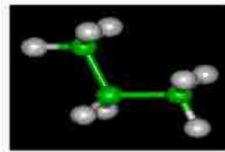
propane C_3H_8
