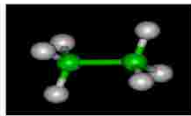
ethane C_2H_6
