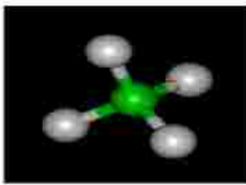
methane CH_4
