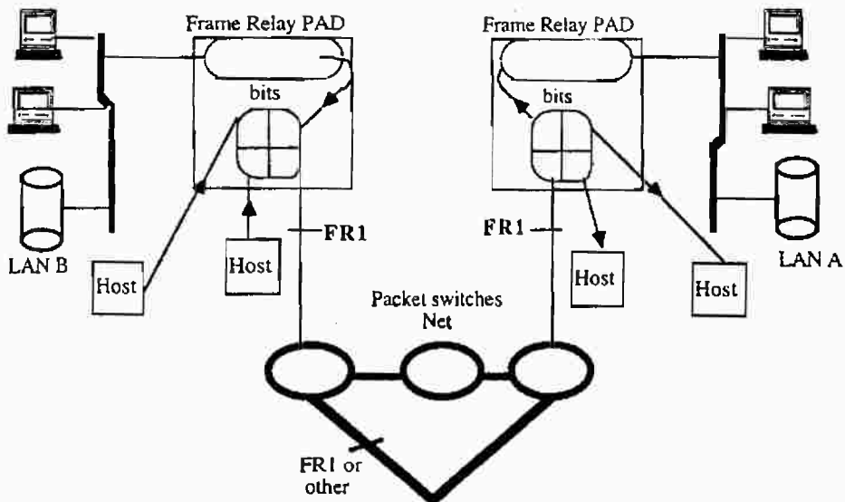
Figure 6: Frame Relay LAN and Host Interconnect.
