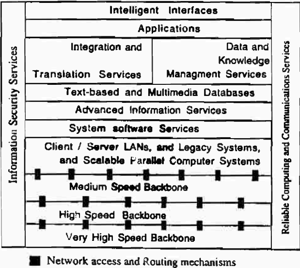
Figure 3: NII hierarchy.
