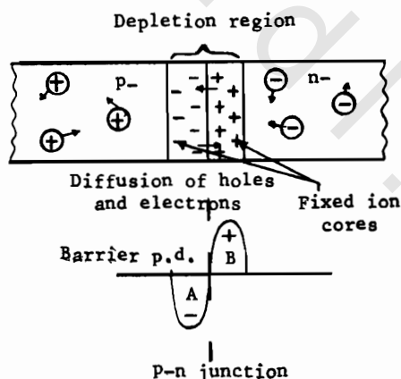
Fig. 3.11. p-n-junction and barrier p.d.
