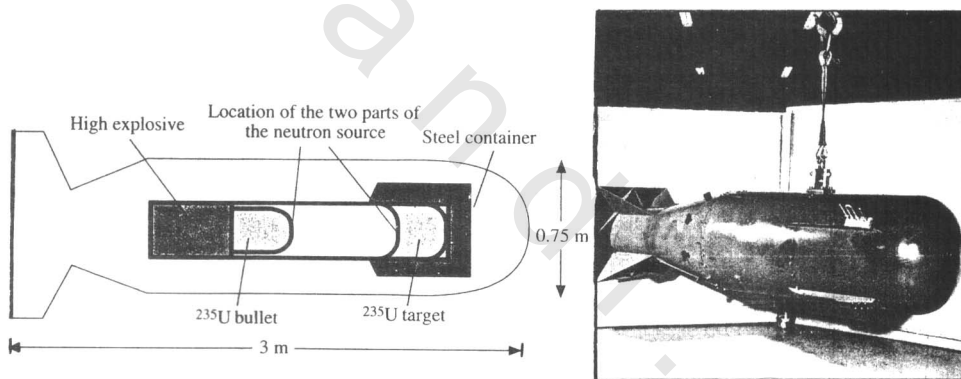
Fig. 3.17. The gun design of the Hiroshima bomb and the bomb dropped on Hiroshima.
