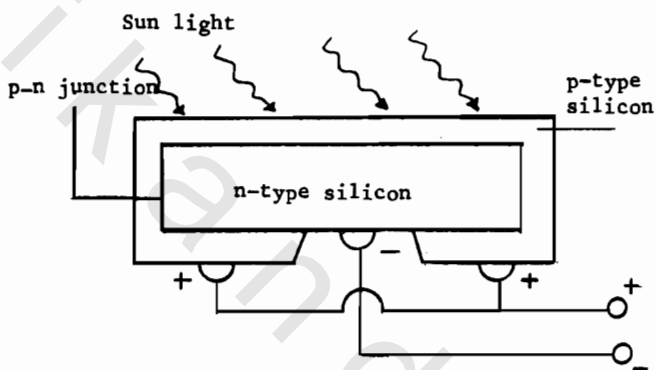
Fig. 3.13. Schematic diagram of a solar cell. The p-side acts as the positive pole of the solar battery.
