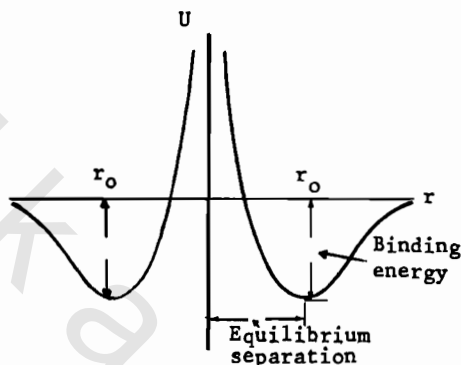
Fig. 3.9. The potential energy curve for a diatomic molecule.
