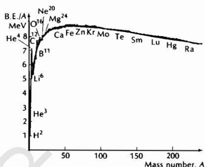
Fig. 3.14. A plot of binding energy per nucleon versus mass number of stable nuclei.
