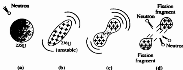
Fig. 3.15. Stages of the fission process of uranium ^{235}\text{U} .
