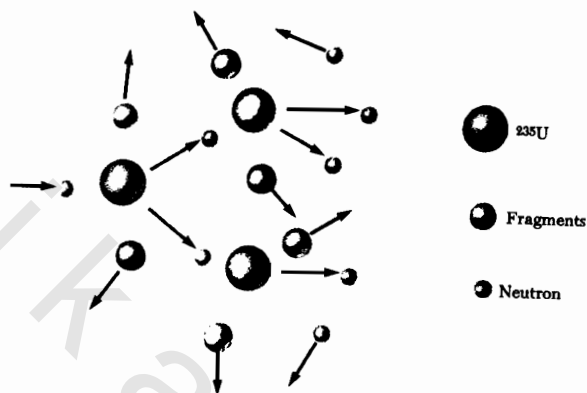
Fig. 3.16. A nuclear chain reaction.
