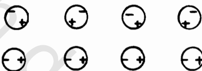
Fig. 3.8. Dipoles in molecular crystals.
