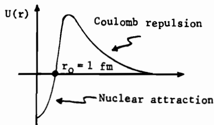
Fig. 3.19. The potential energy as a function of separation between two nuclei. The two nuclei require energy greater than the height of the barrier to undergo fusion.
