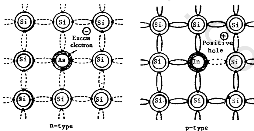
Fig. 3.10. n- and p- semiconductors.
