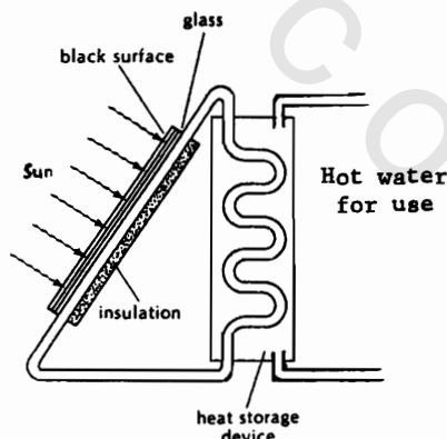
Fig. 3.4. Scheme of a solar water heater.
