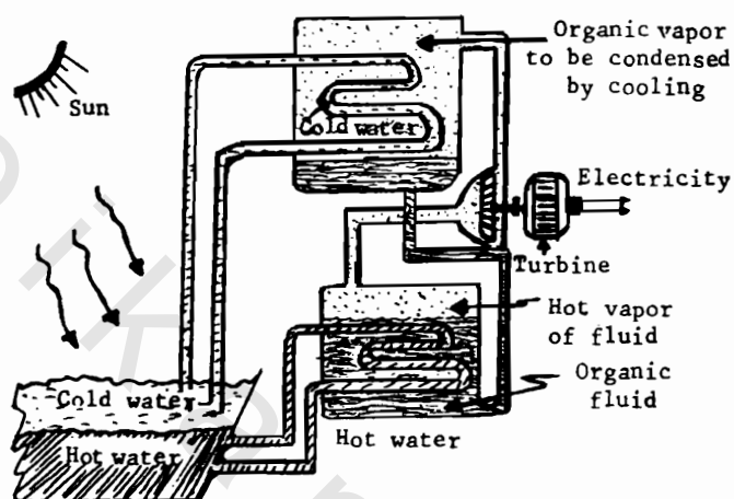
Fig. 3.7. A schematic diagram of a solar pond power station.
