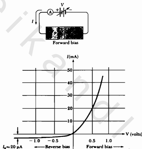
Fig. 3.12. The characteristic curve for a real diode.
