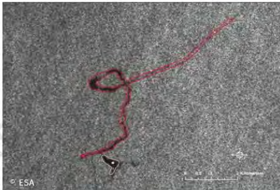
Figure 3.8: Possible seepage slicks identified offshore Indonesia (Biegert, 2007).
