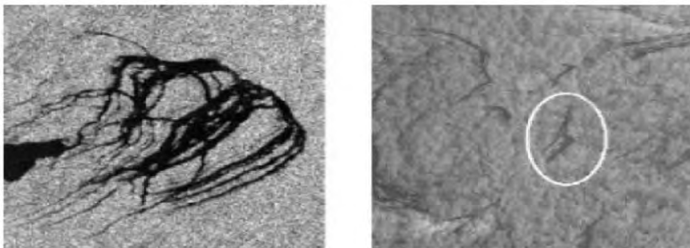
Figure 3.7: Direct detection of hydrocarbon seeps using radar imagery (Biegert, 2007).
