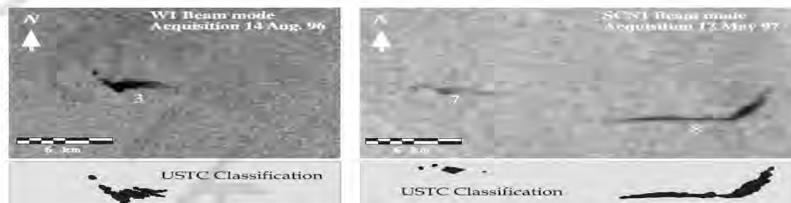
Figure 3.4. Examples of seepage slicks identified on RADARSAT-1 SCN1 and W1 images and corresponding USTC classification results.
