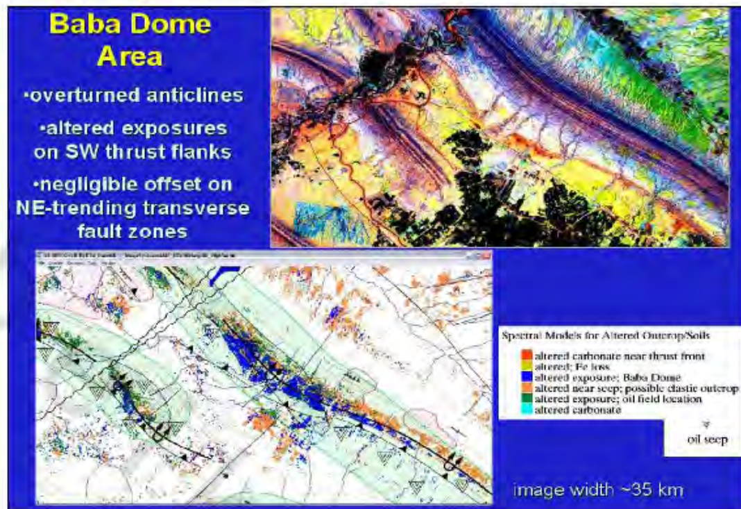
Figure 3.10: Enhanced Landsat image of the Baba Dome portion of the Kirkuk oil field. (Sandra et al, 2011)
