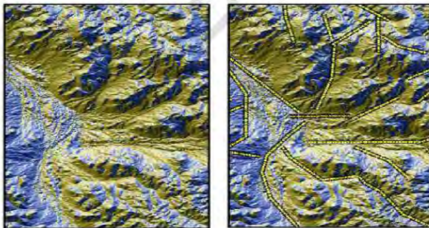
Figure 3.12. Slope direction image of a 200km 2 area in western Libya (Sandra et al, 2011).
