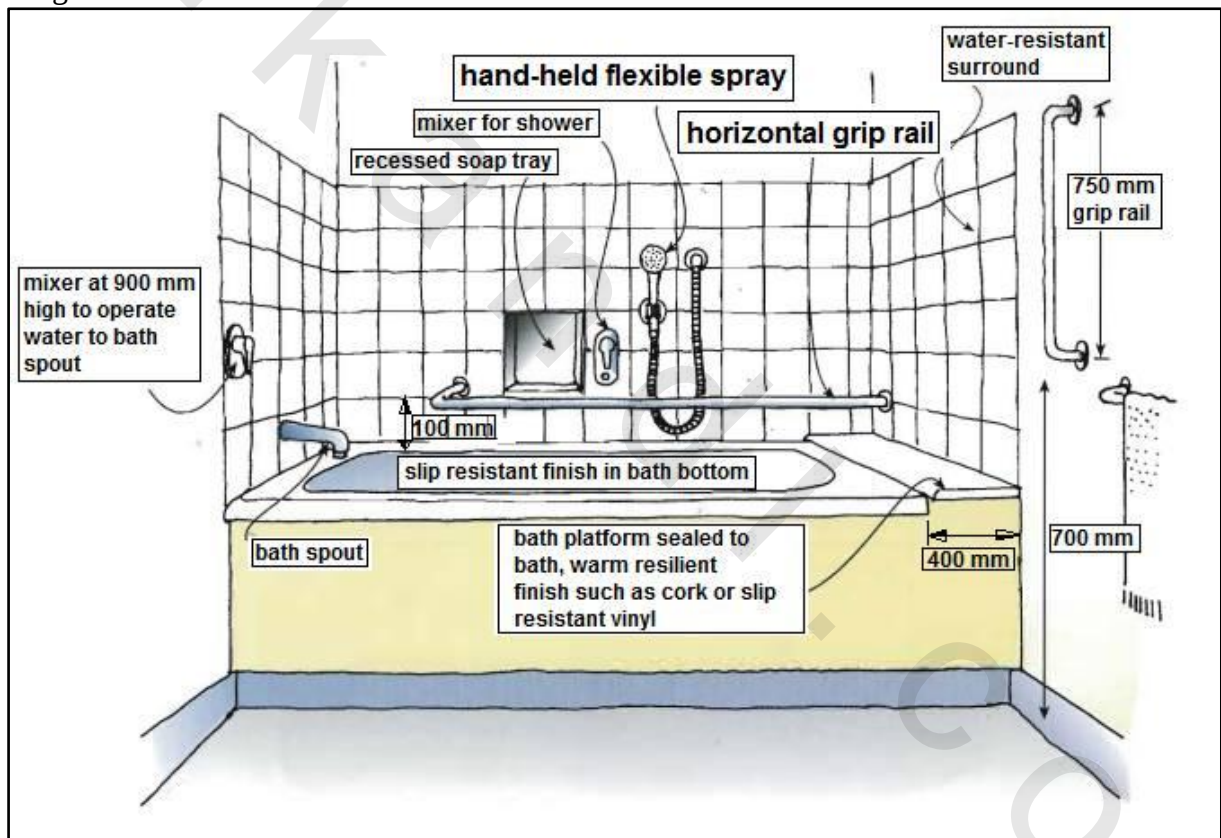
Figure 5-27 Combination bath and shower that may suit some wheelchair-users
