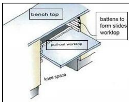
Figure 5-47 Pull-out adjustable height worktop
