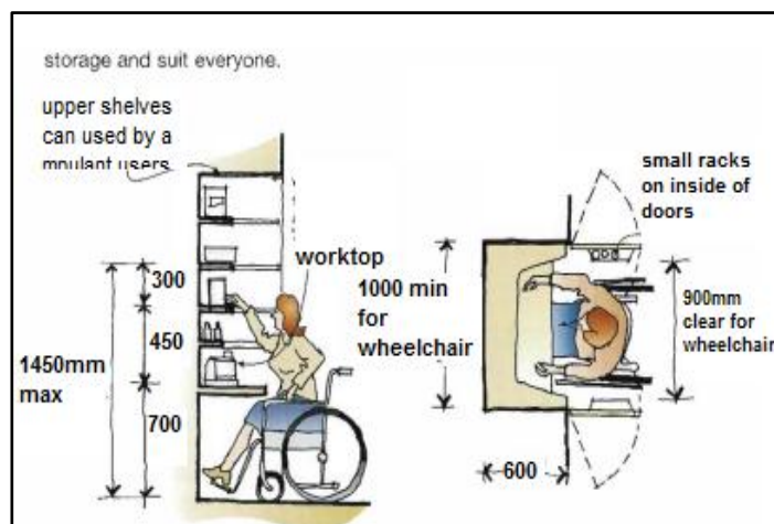
Figure 5-57 A walk-in or wheel-in pantry
