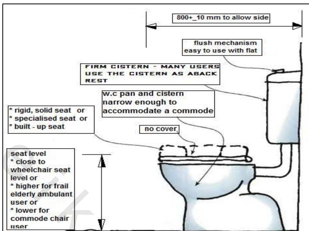
Figure 5-19 Desirable features in a toilet
