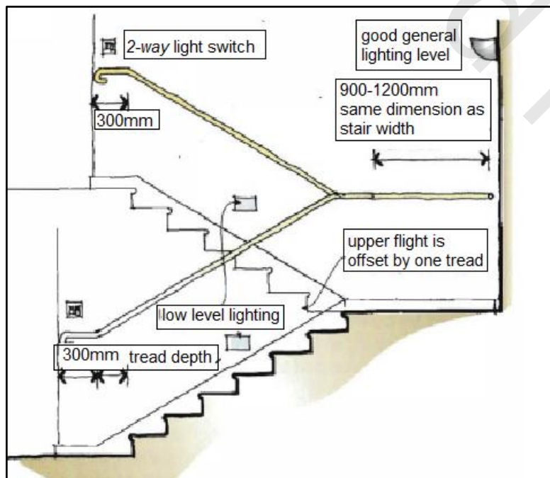
Figure 5-9 Stairs with a lighting
