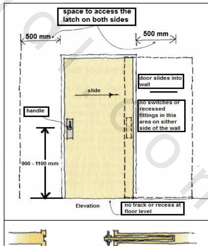
Figure 5-72 A cavity sliding door
