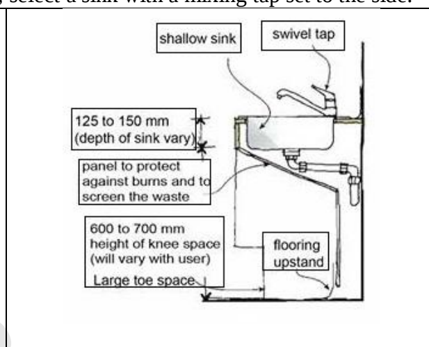
Figure 5-53 Knee-space underneath a sink provides for wheelchair access
