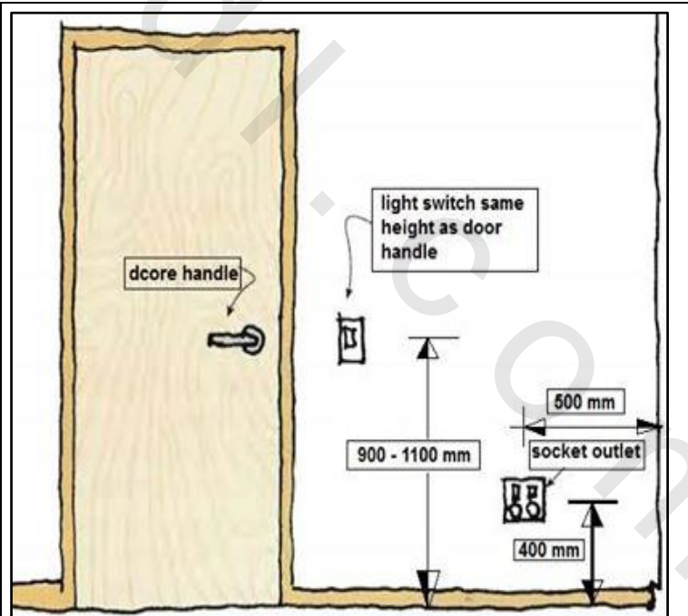
Figure 5-34 Preferred positions of light switches and socket
