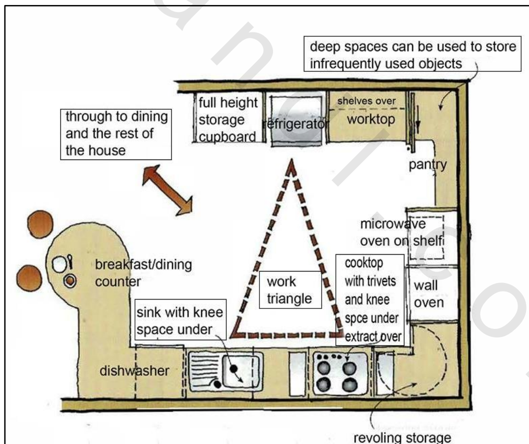
Figure 5-42 U -shaped kitchen layout
