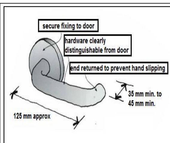
Figure 5-74 User-friendly lever handle
