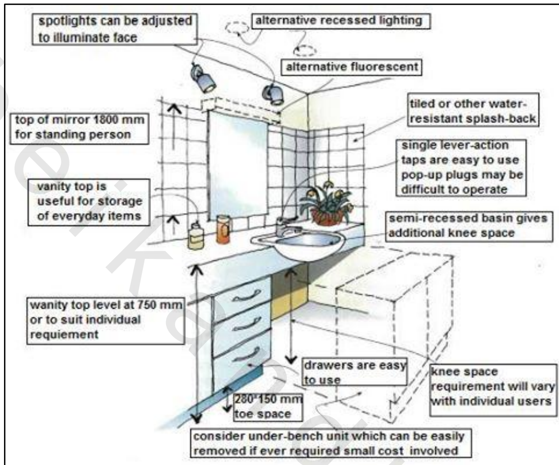
Figure 5-22 Removable vanity modules make knee-space available
