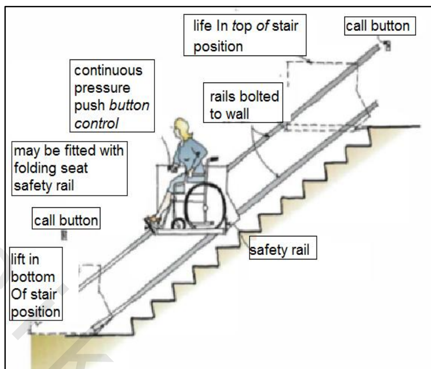
Figure 5-11 Features of a wheelchair platform lift
