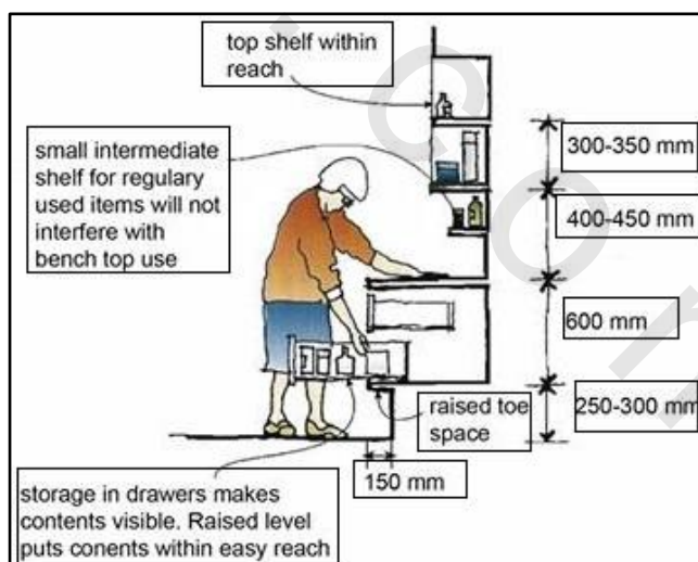
Figure 5-54 Indicates the range of storage suitable for most adults
