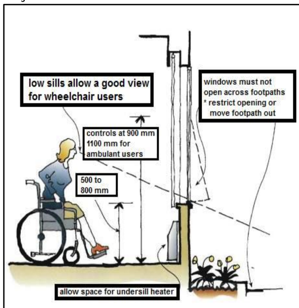
Figure 5-76 Garden keeps people at safe distance from protruding window
