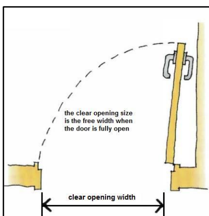
Figure 5-66 Clear opening width
