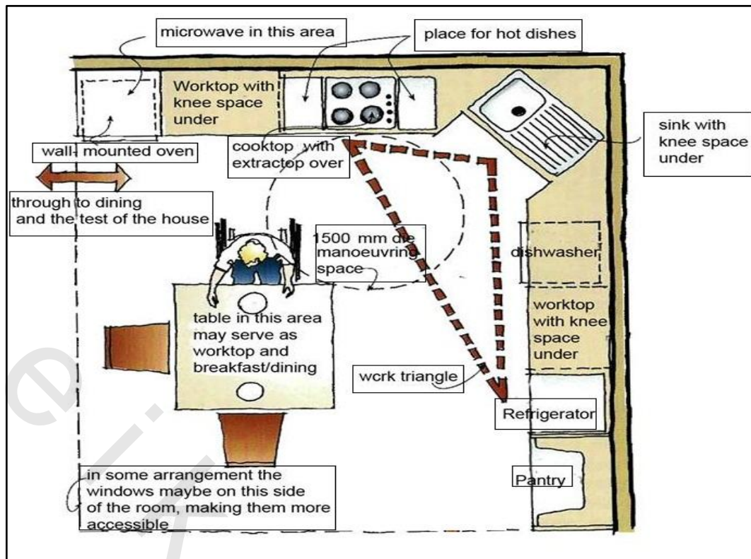
Figure 5-41 L --shaped kitchen
