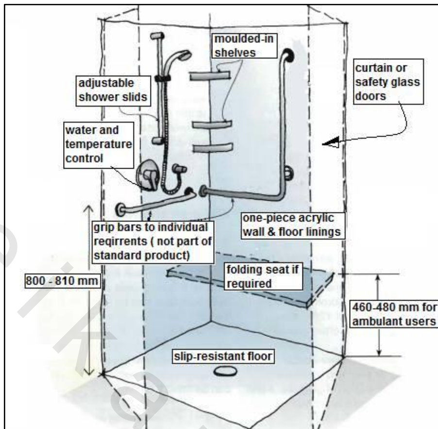
Figure 5-28 Wet area shower with no raised hob
