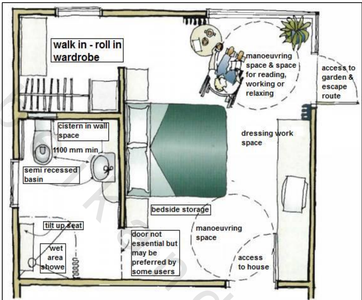
Figure 5-31 A double access-friendly bedroom
