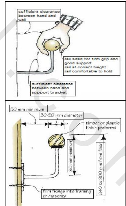
Figure 5-10 Comfortable handrail design
