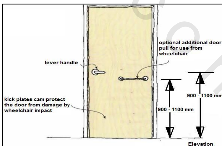
Figure 5-67 Hinged door layout
