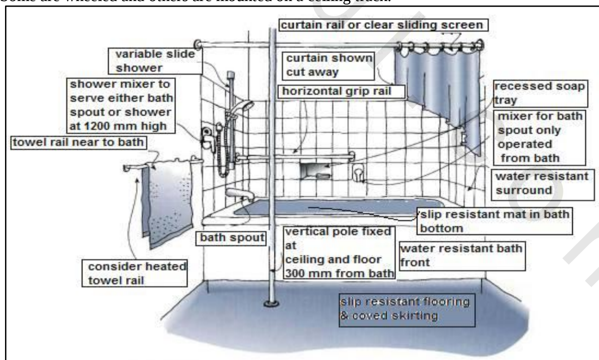
Figure 5-25 A combination bath and shower with additions designed to make it more accessible
