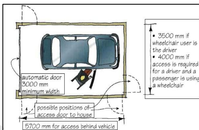
Figure 5-2 A minimal garage layout
