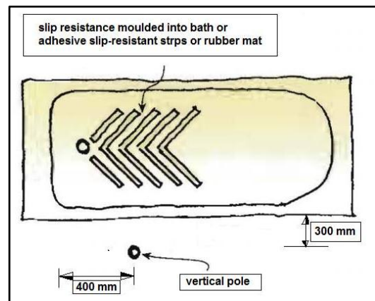
Figure 5-26 Slip-resistant adhesive
