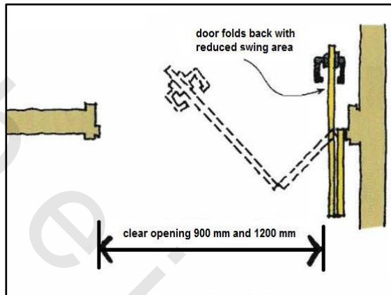
Figure 5-70 A bi-fold door
