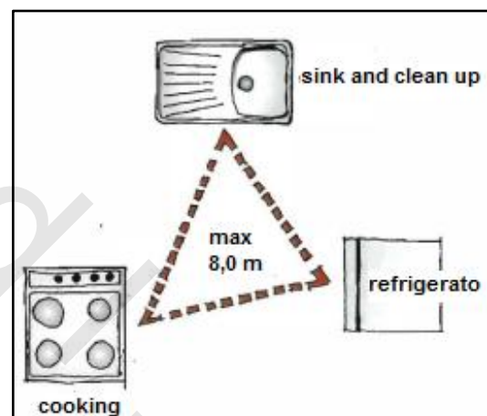
Figure 5-40 Locating the kitchen fittings for easy use
