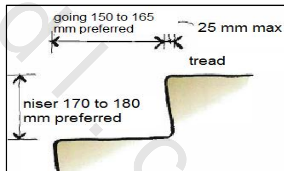
Figure 5-6 Step dimensions
