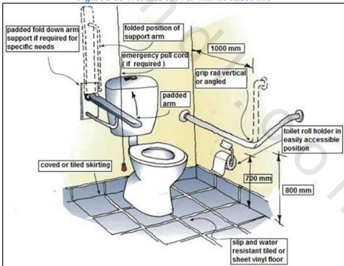
Figure 5-29 Grabrails make it easier to access bathroom fittings
