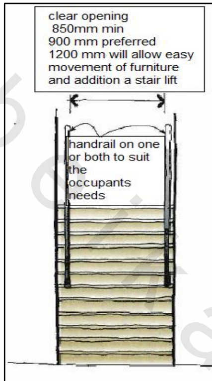
Figure 5-7 Width of a stair
