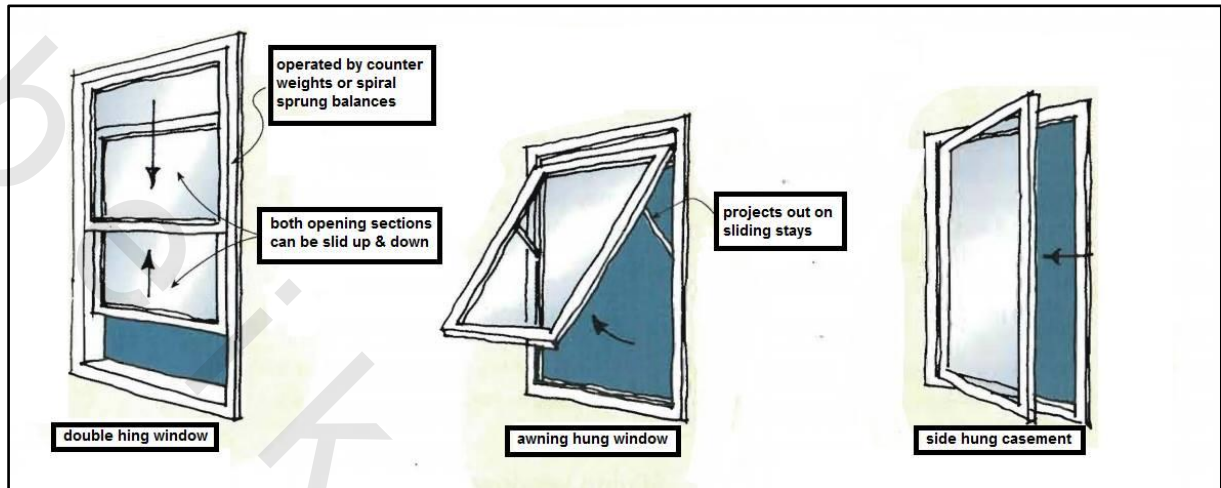
Figure 5-75 Window options: double hung sash, awning hung and casement sash
