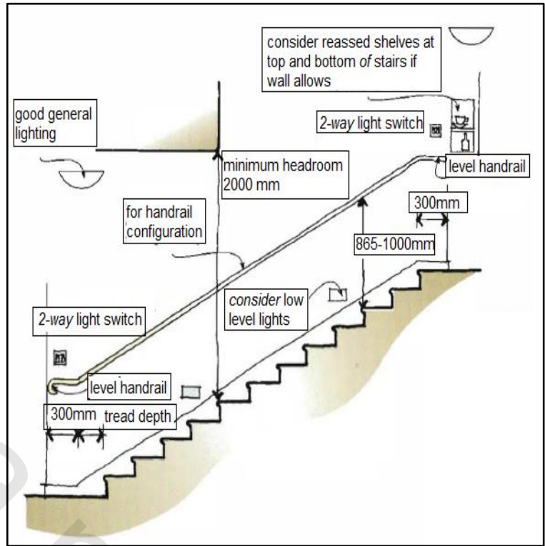
Figure 5-8 A straight of stairs
