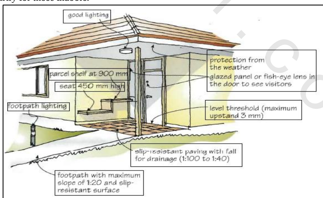
Figure 5-1 Elements of an accessible entrance
