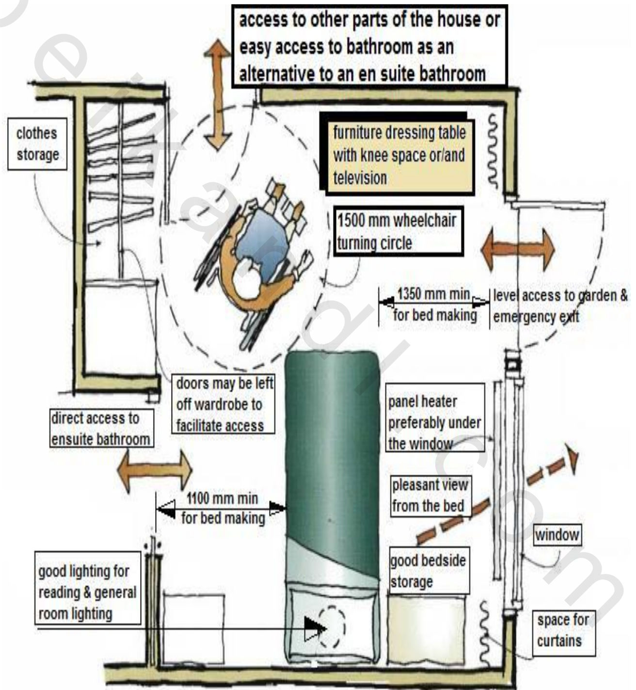
Figure 5-30A single access-friendly bedroom
