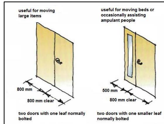
Figure 5-71 Some double door
