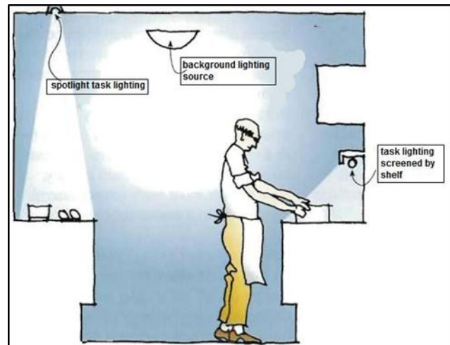
Figure 5-32 Background lighting and task lighting.
