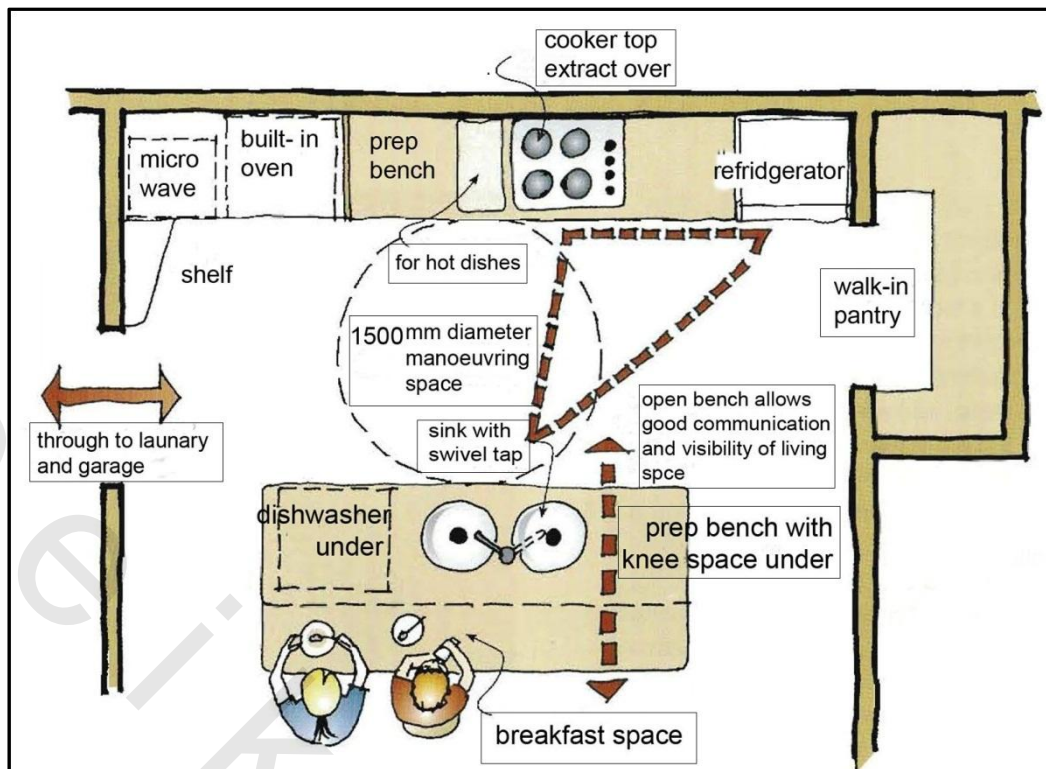
Figure 5-43 A galley plan kitchen
