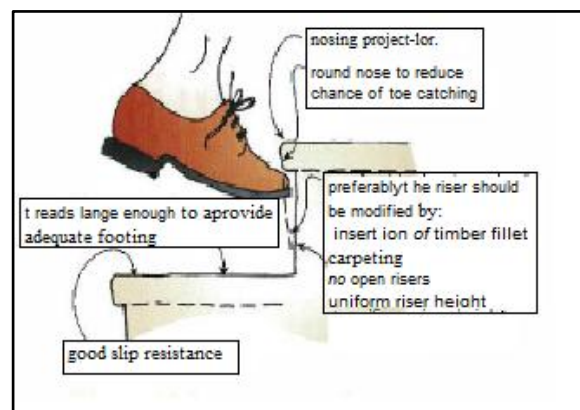
Figure 5-5 Principles of step design
