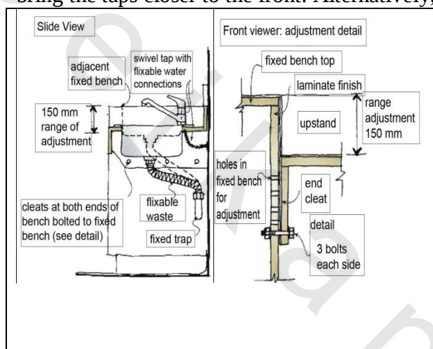
Figure 5-52 An adjustable height sink
