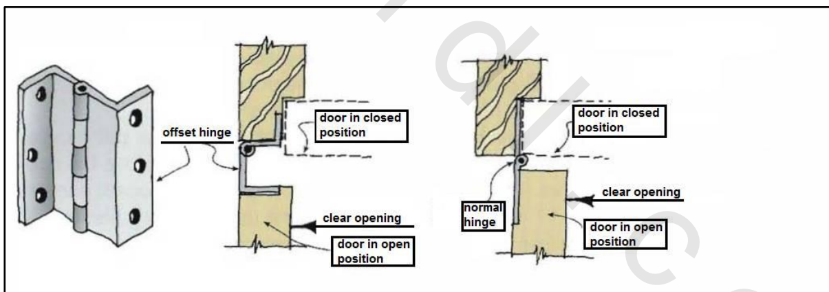
Figure 5-69 Offset hinge
