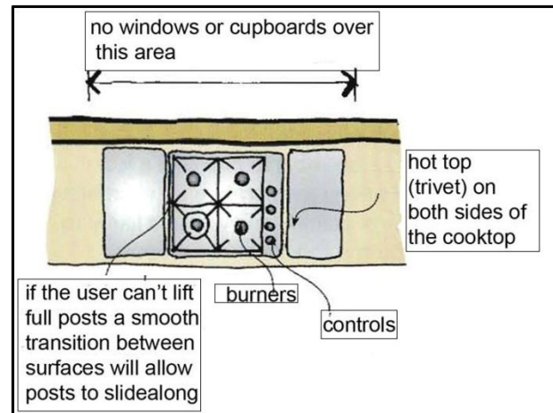
Figure 5-62 Layout of a Cook-top
