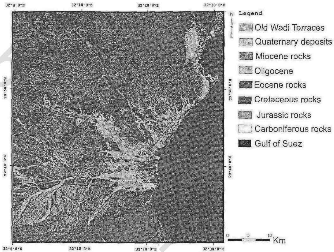
Figure (14): Landsat ETM+ image supervised classification.
