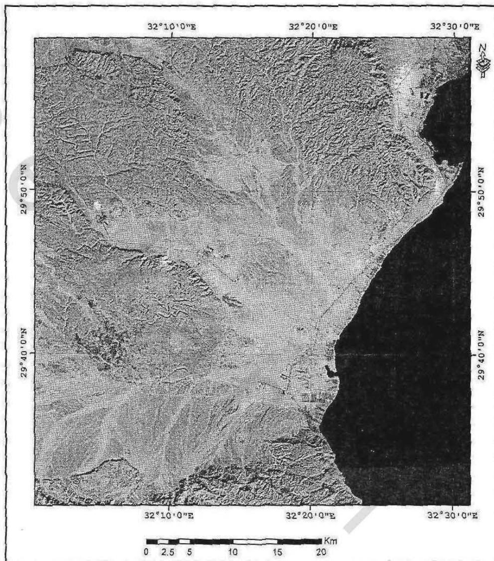
Figure (7): False color composite Landsat ETM+ image (7, 4, 2) in RGB, of the study area.
