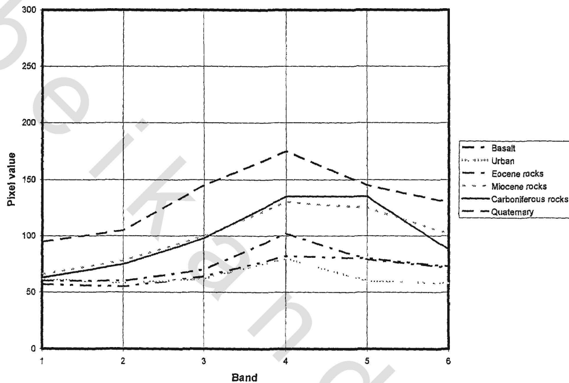
Figure (5): The spectral reflectance curves for some common rock types cover the study area.
