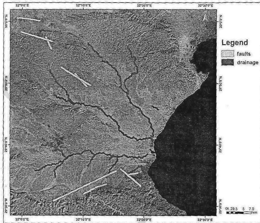
Figure (88): Risk map showing the buffer zone of active faults and drainage basin.
