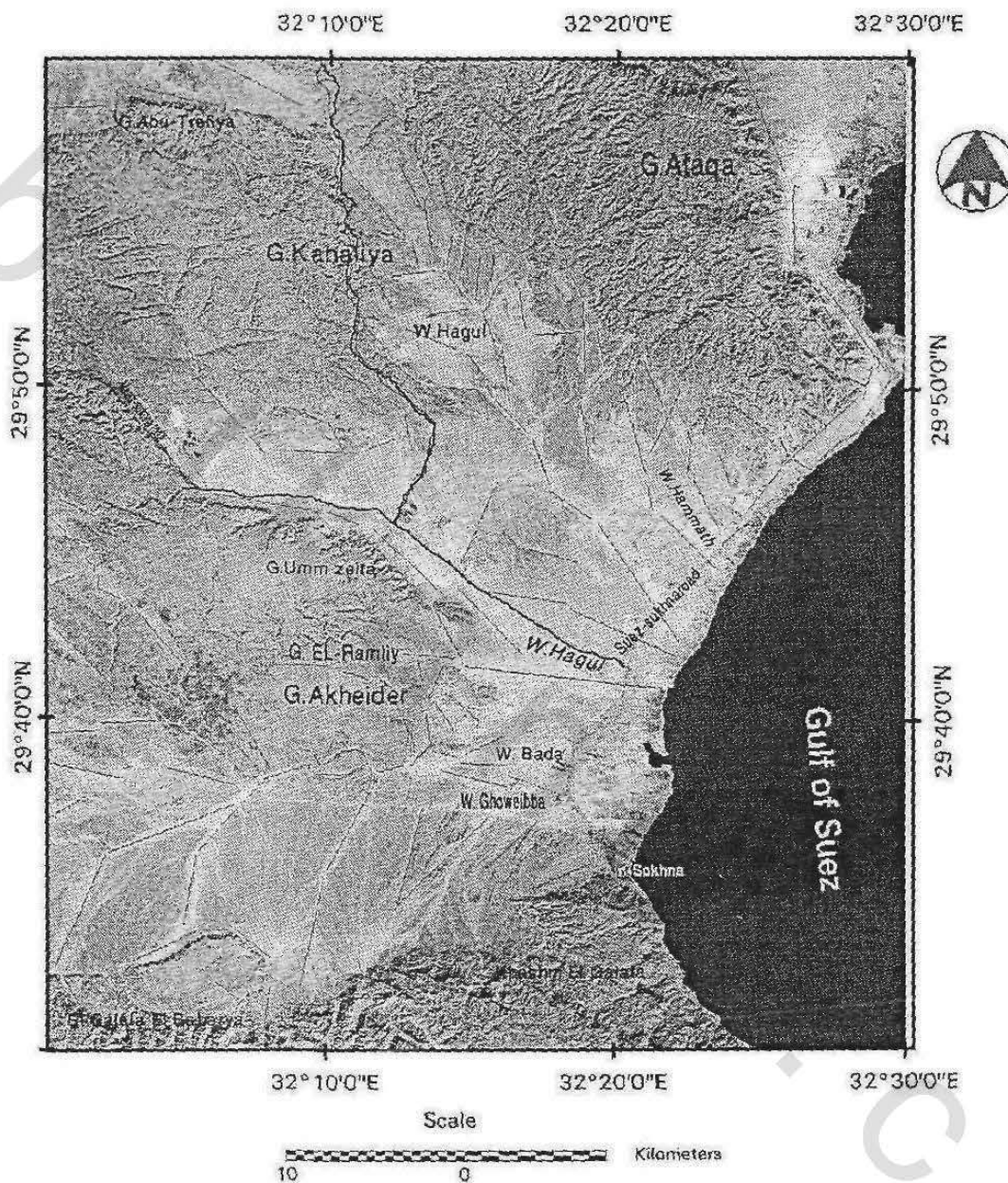
Figure (77): Lineaments map of the study area extracted from the Landsat image.
