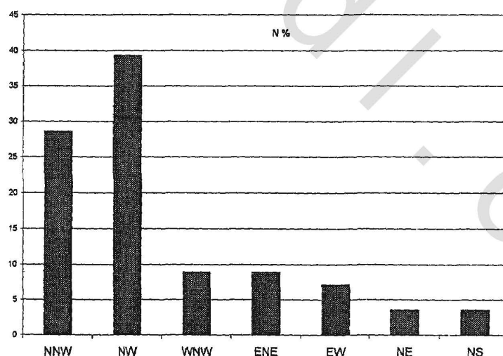
Figure (80): Histogram showing the structural extracted from geological map.
