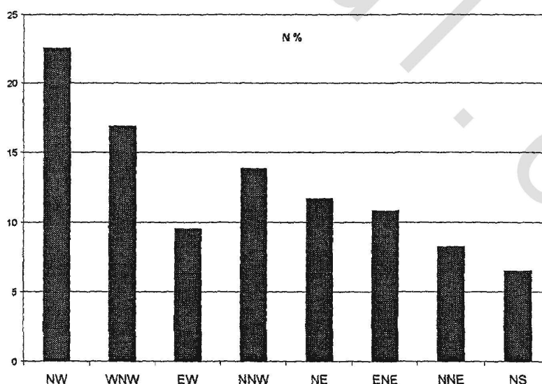
Figure (79): Histogram showing the structural trends of lineaments traced from ETM+ image.
