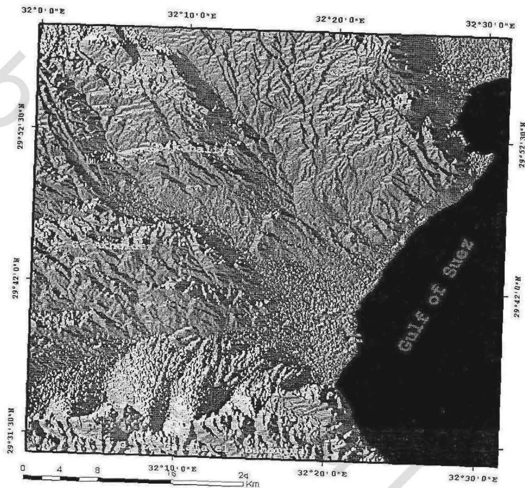
Figure (76): Shaded relief map of the study area.
