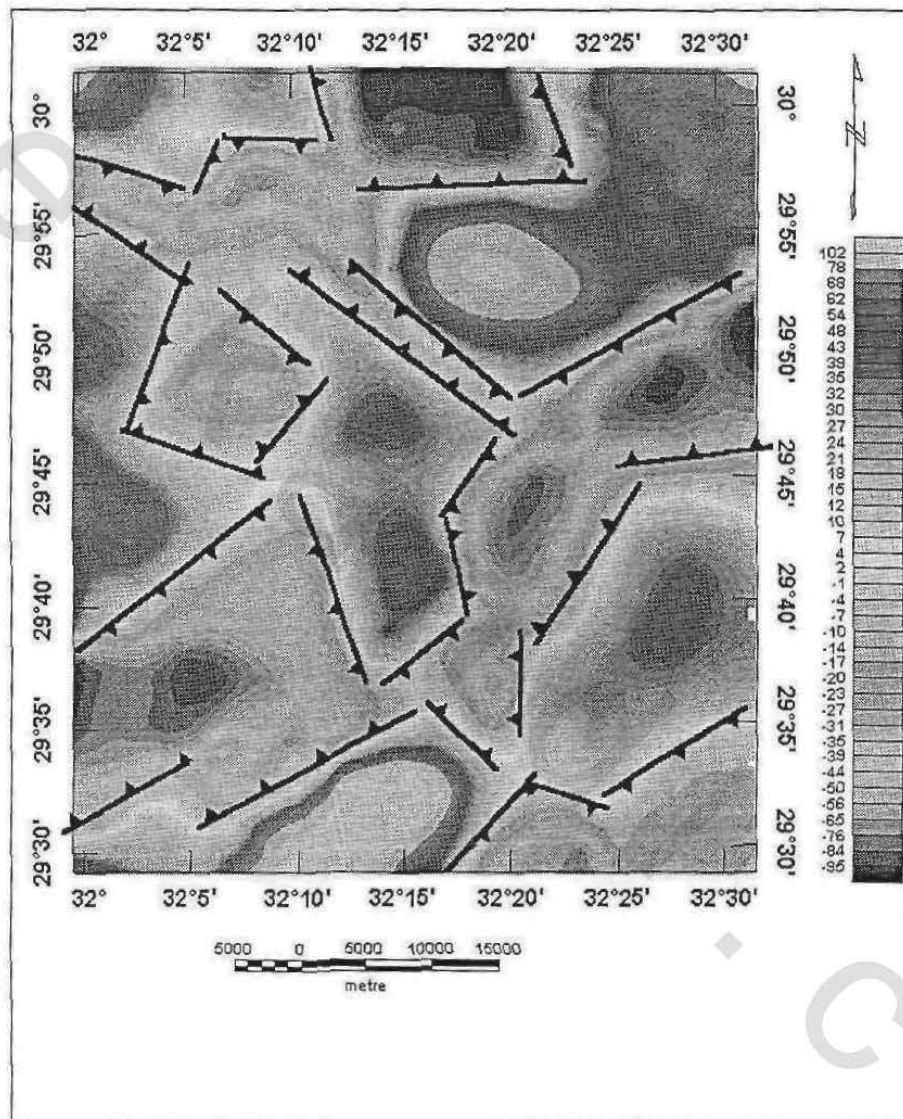
Figure (81): Fault elements dissecting the study area from magnetic interpretation.
