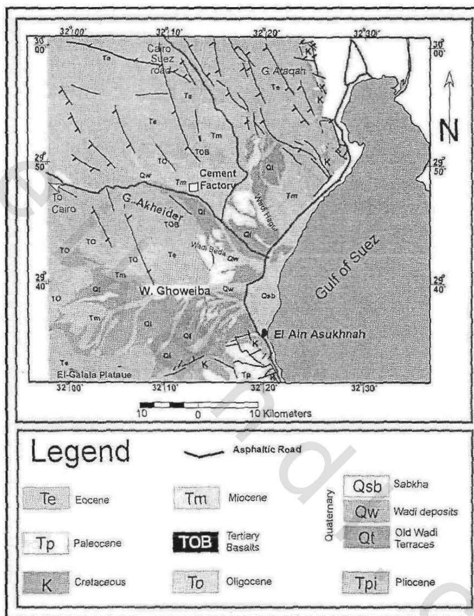
Figure (78 ) Geological map of the study area (after EGSM,1999).
