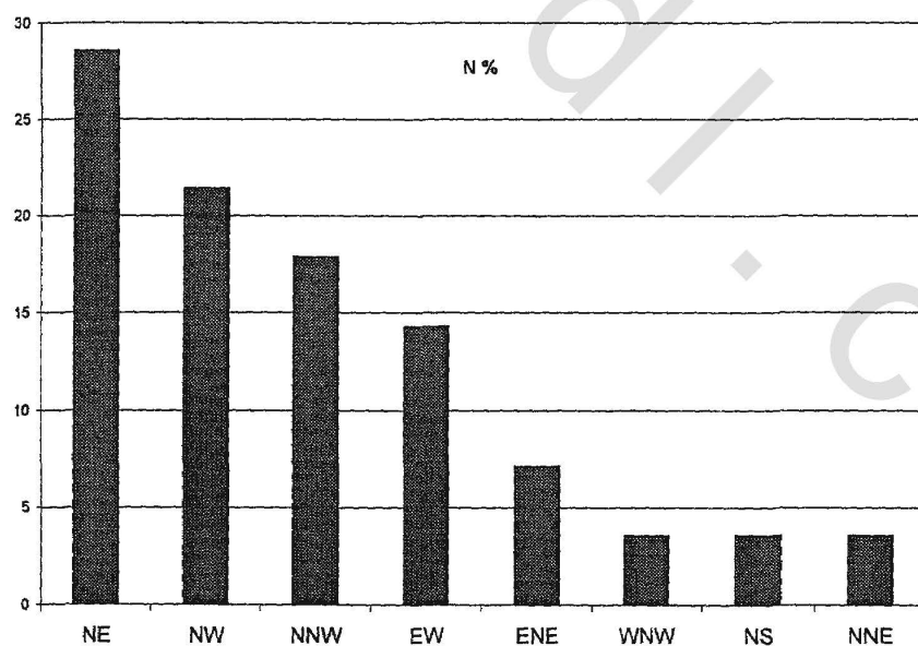
Figure (82): Histogram showing the main structural trends extracted from magnetic map.
