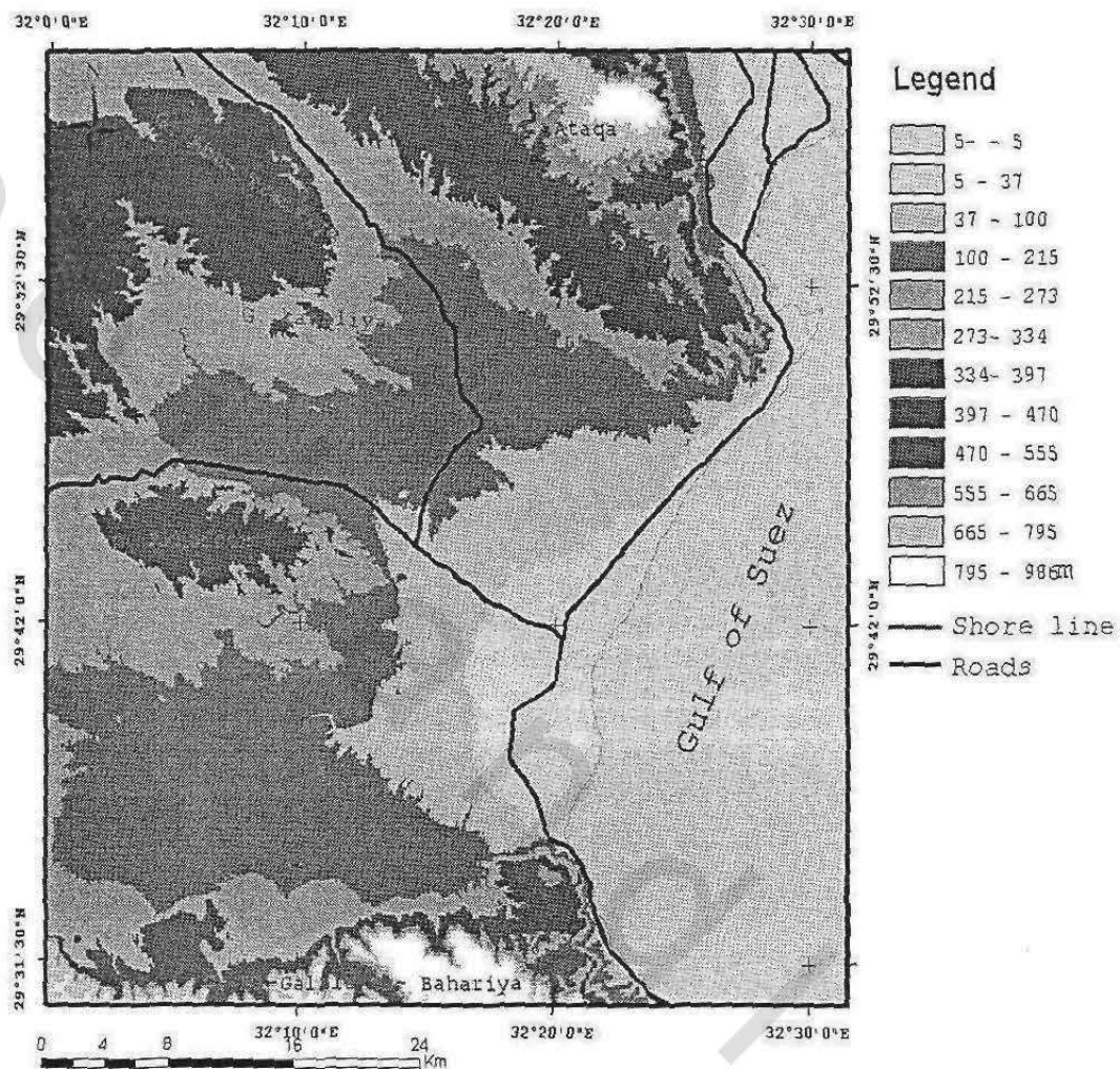
Figure (74): Digital Elevation Model (DEM) of the study area.
