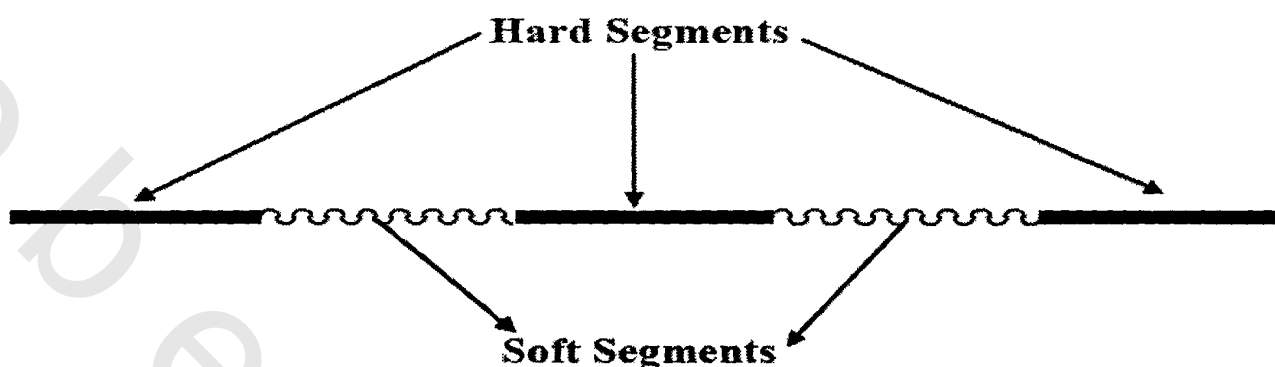
Figure 1: Schematic representation of segmented polyurethane.
