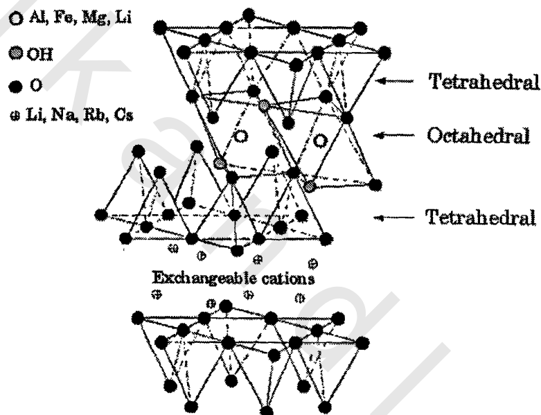
Figure 4: Structure of 2:1 phyllosilicates
