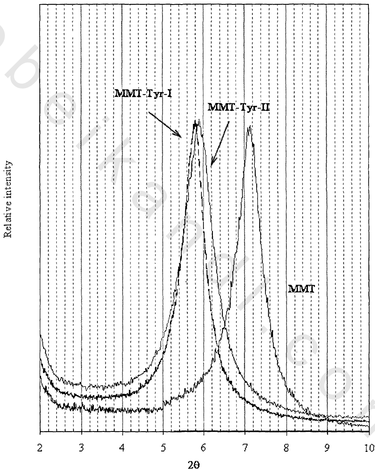
Figure 24 : The X-ray diffraction patterns of Tyr – MMT ( I_a ) first and second treatmen
