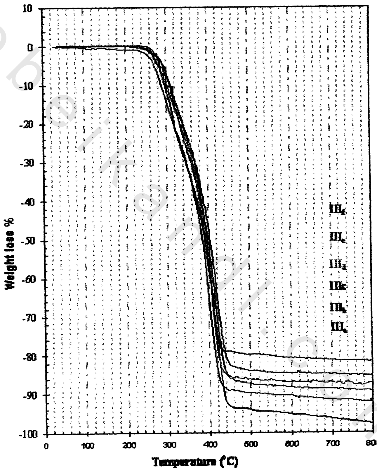
Figure 11: TGA thermographs under argon atmosphere for PU-organoclay composites III_{n,4} (Tyr-MMT)
