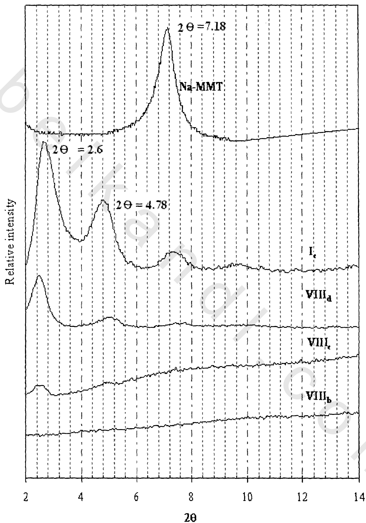
Figure 28: XRD pattern for Na-MMT, I_t and VIII_{b-d}
