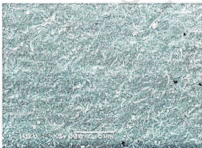
Figure 33b: SEM micrograph of PU/ SMA- ALA-MMT, 10 wt. % ( V_d )
