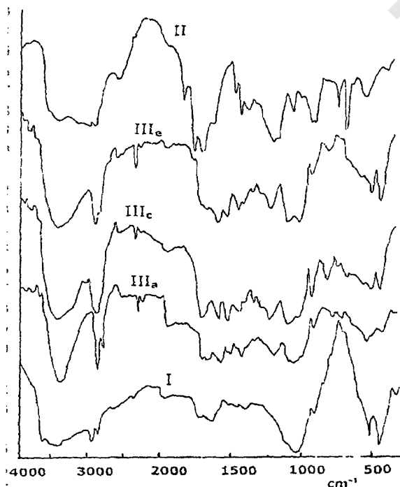
Figure 1. IR spectra for organoclay I, copolymer II and PU-organoclay III a,e .
