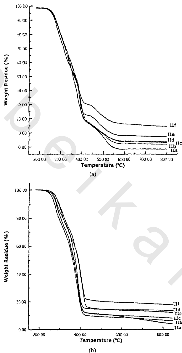
FIG. 2. (a) TGA thermograms for PU-organoclay samples (from down to top II a , II b , II c , II c , II e , and II f ) in air. (b) TGA thermograms under argon atmosphere for PU-organoclay composites II a-f .
