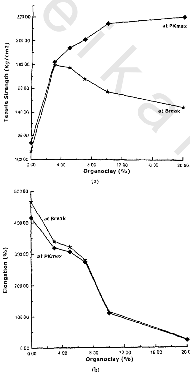
FIG. 6 (a) Tensile strength for PU-tyr-MMT nanocomposites II a-f at PK max and at break. (b) Elongation for PU-tyr-MMT nanocomposites II a-f at PK max and at break.
