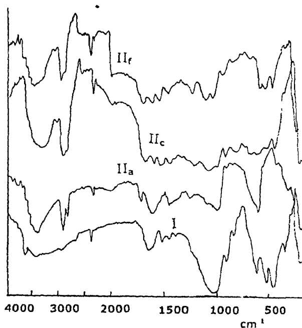
FIG. 1. IR spectra for organoclay I and PU-Tyr-MMT \text{II}_{a..r} .
