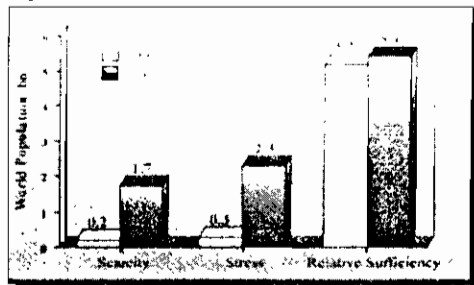
figure 2.2 Access to fresh water 1995 2050
