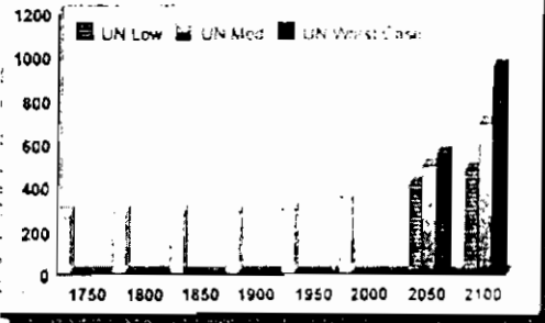
Figure 2.1 Carbon Dioxide
