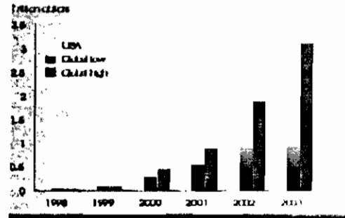
Figure 2.6 Projected Internet Commerce
