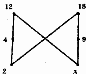
(و) (\{2, 3, 4, 9, 12, 18\}, |)
