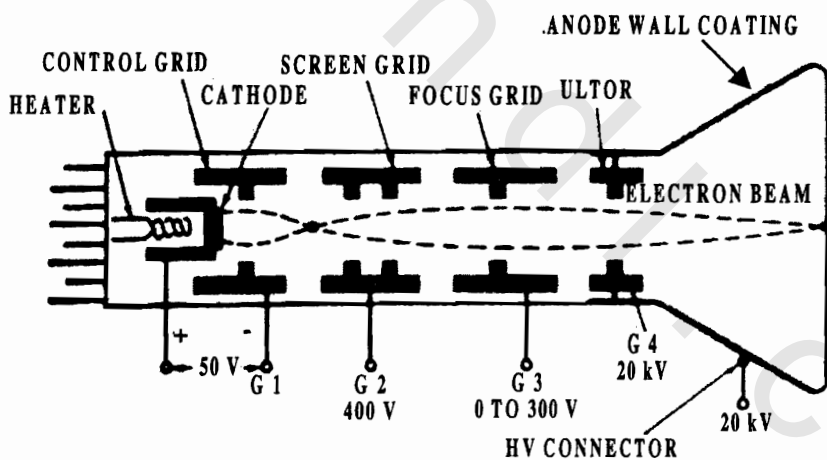
Fig. 12.18 Structure of electron gun with electronic focusing and magnetic deflection
