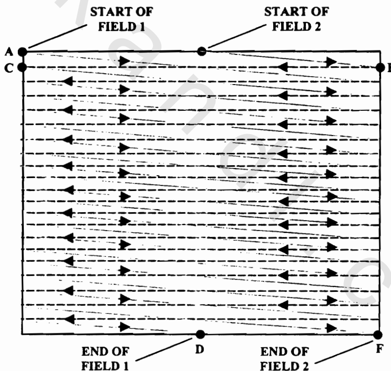
Fig. 12.4 Interlacing
