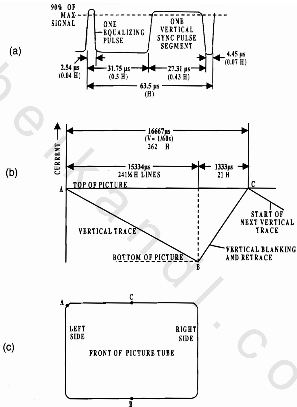
Fig. 12.7 Vertical retrace
