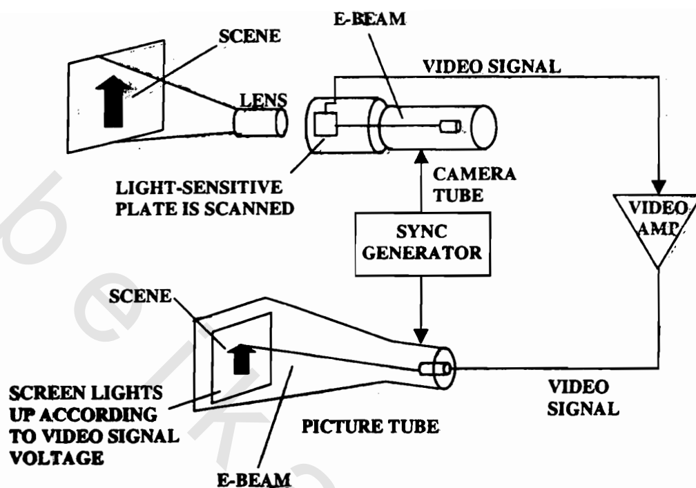
Fig. 12.2 A simplified TV system (camera and receiver)
