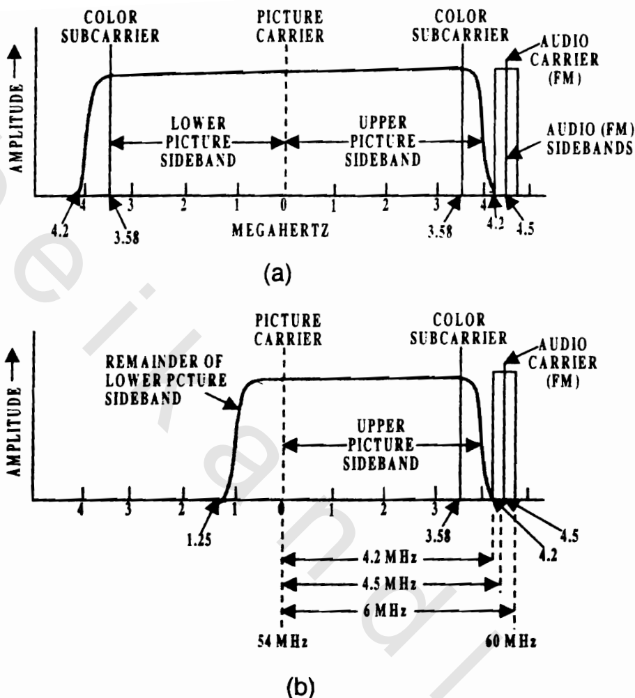
Fig. 12.16 Frequency spectrum of composite TV signal a) DSB b) VSB
