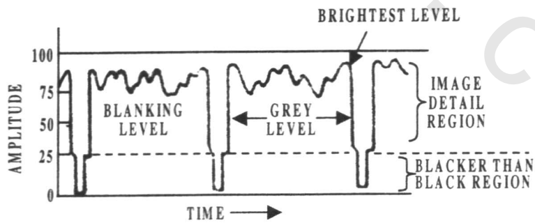
Fig. 12.15 Positive picture phase
