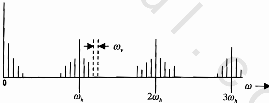
Fig. 12.13 Spectrum of a monochrome video signal
