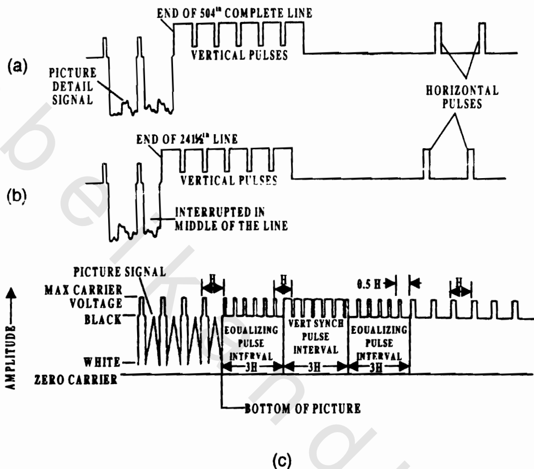
Fig. 12.10 The form of video signal
