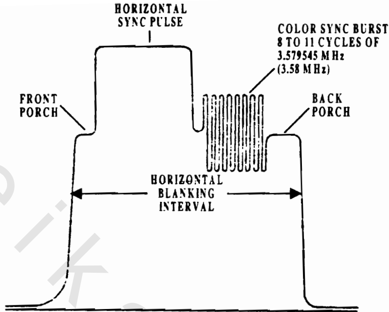
Fig. 12.11 Color burst signal
