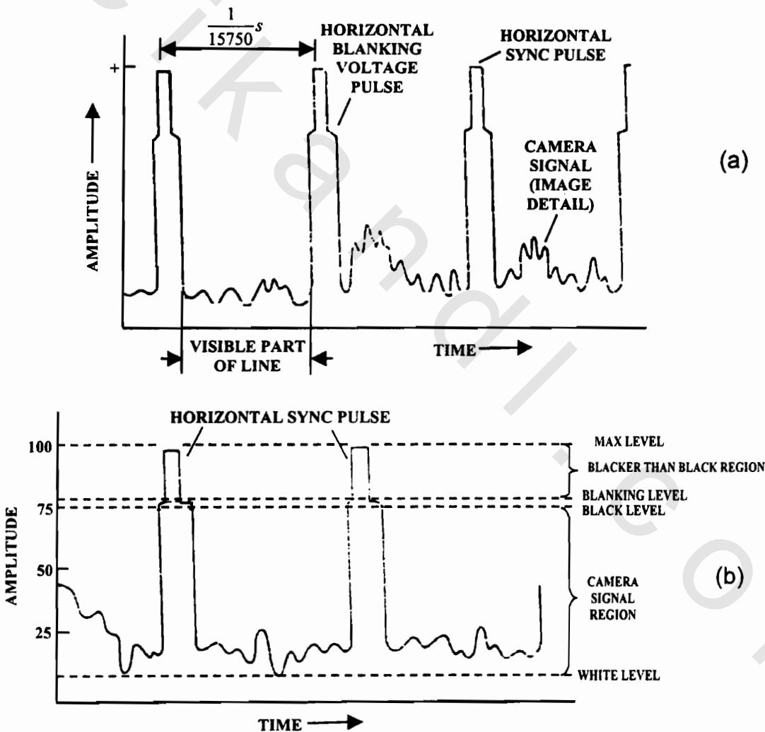
Fig. 12.5 Composite video signal including blanking and sync pulses a) waveform b) signal levels
